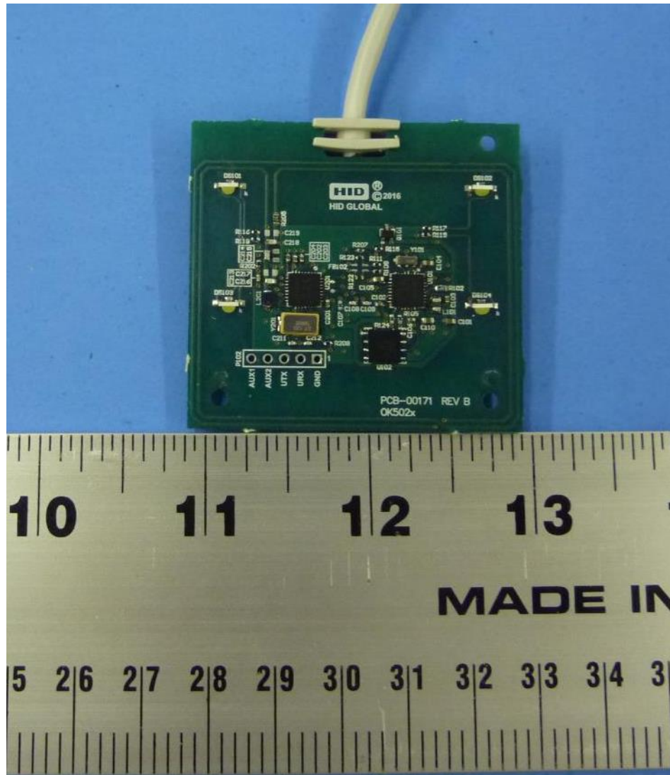
Figure 1: Photo of RFID Reader (Top View)
