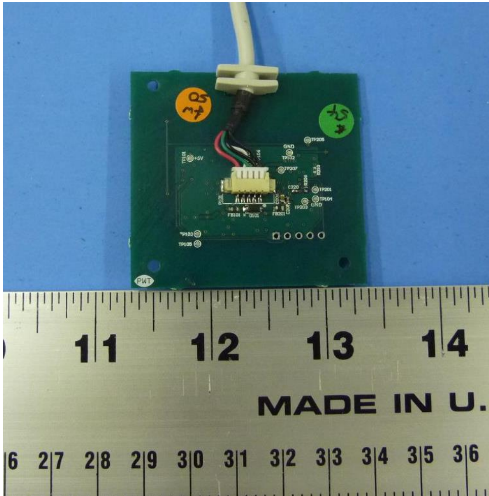
Figure 2: Photo of RFID Reader (Bottom View)
