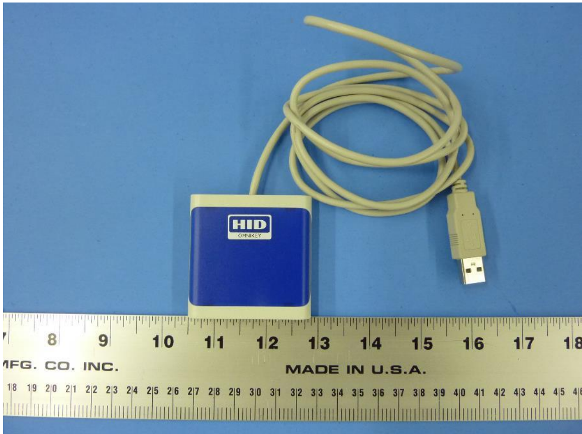
Figure 1: Photo of RFID Reader (Top View)
