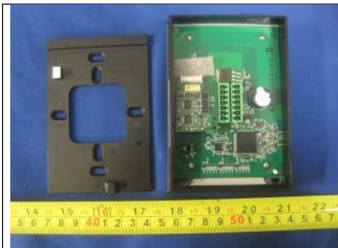
Cover Off View (Terminal Connector)
