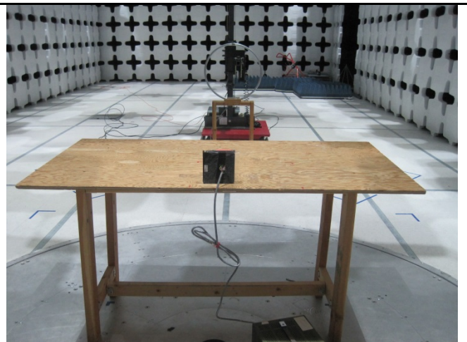
Radiated Emission Test setup (<30MHz) - Rear
