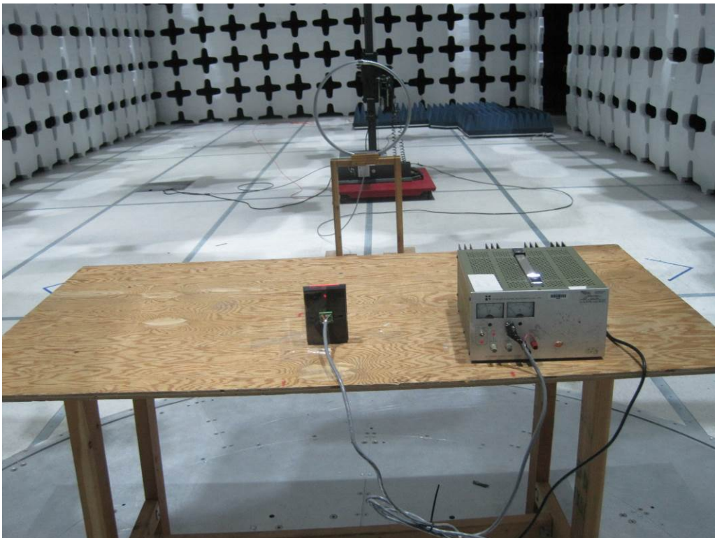
Radiated Emissions (<30MHz) – Rear View
