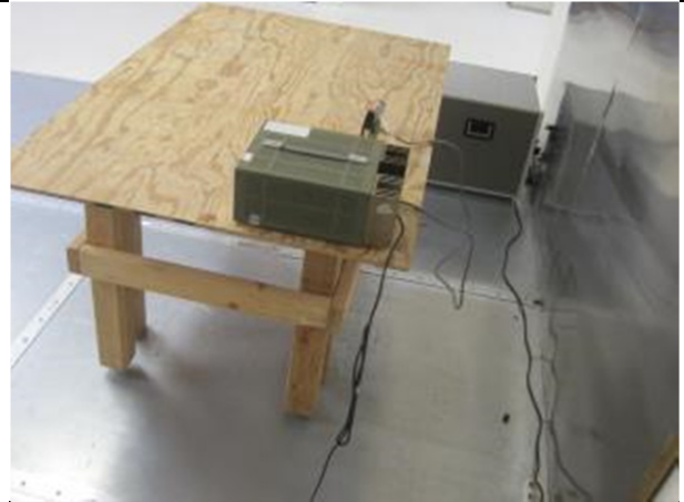
Conducted Emissions Test setup – Rear View
