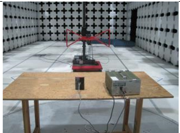
Radiated Emissions Test setup (<1GHz) – Rear View
