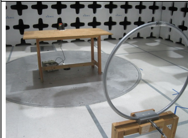
Radiated Emission Test setup (<30MHz) - Front
