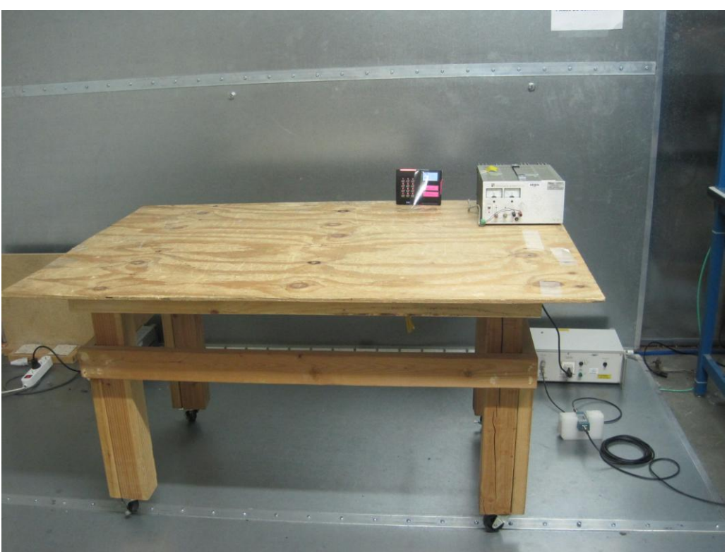
Conducted Emission Test Setup – Front View (Terminal Connectors)
