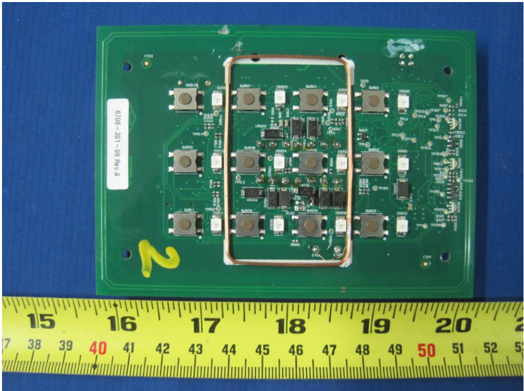
RPKCL40A Terminal Back View
