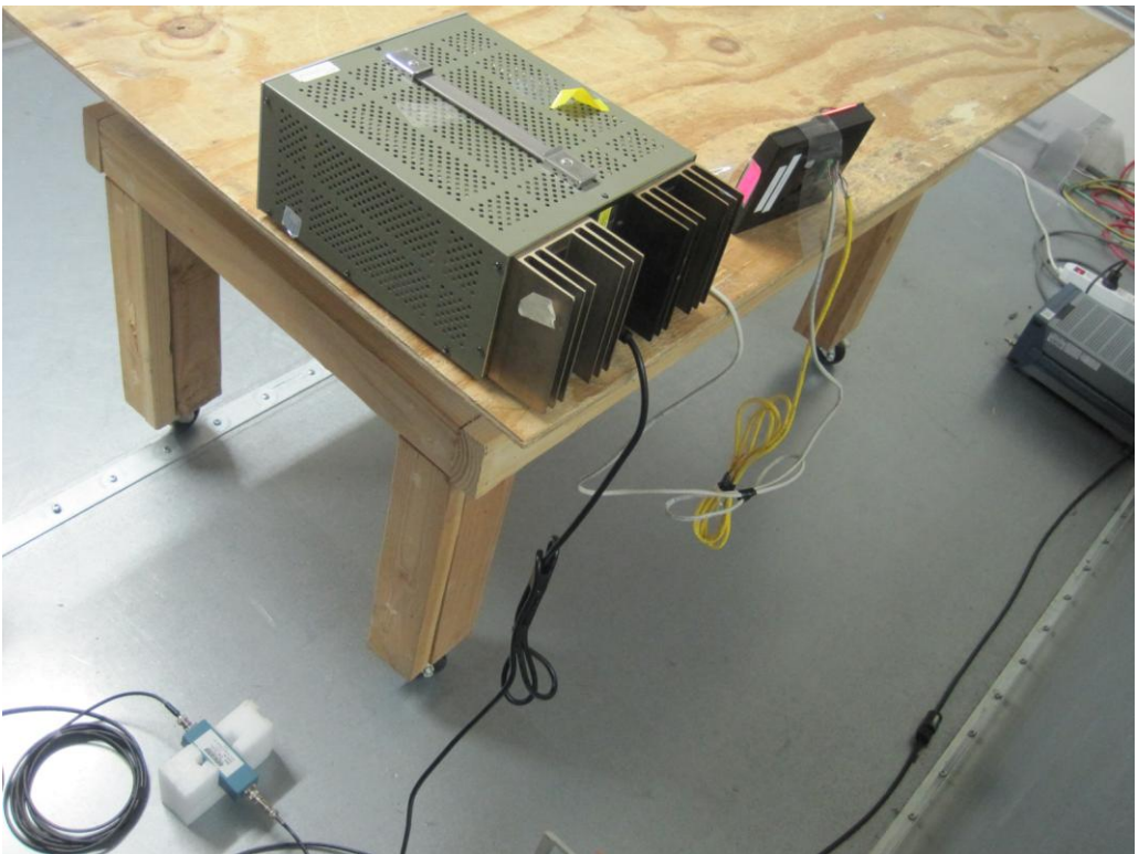
Conducted Emission Test Setup – Rear View (Terminal Connectors)
