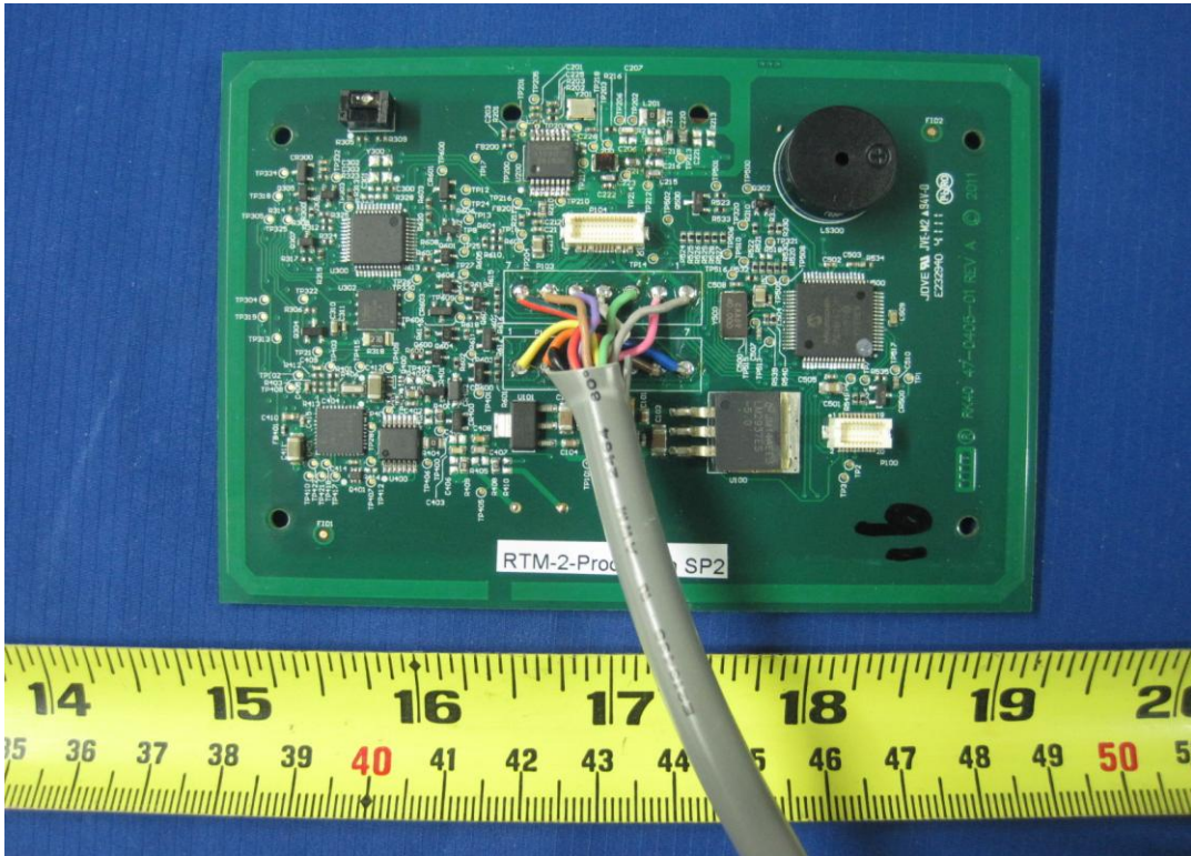
RPKCL40A Pig Tail Front View
