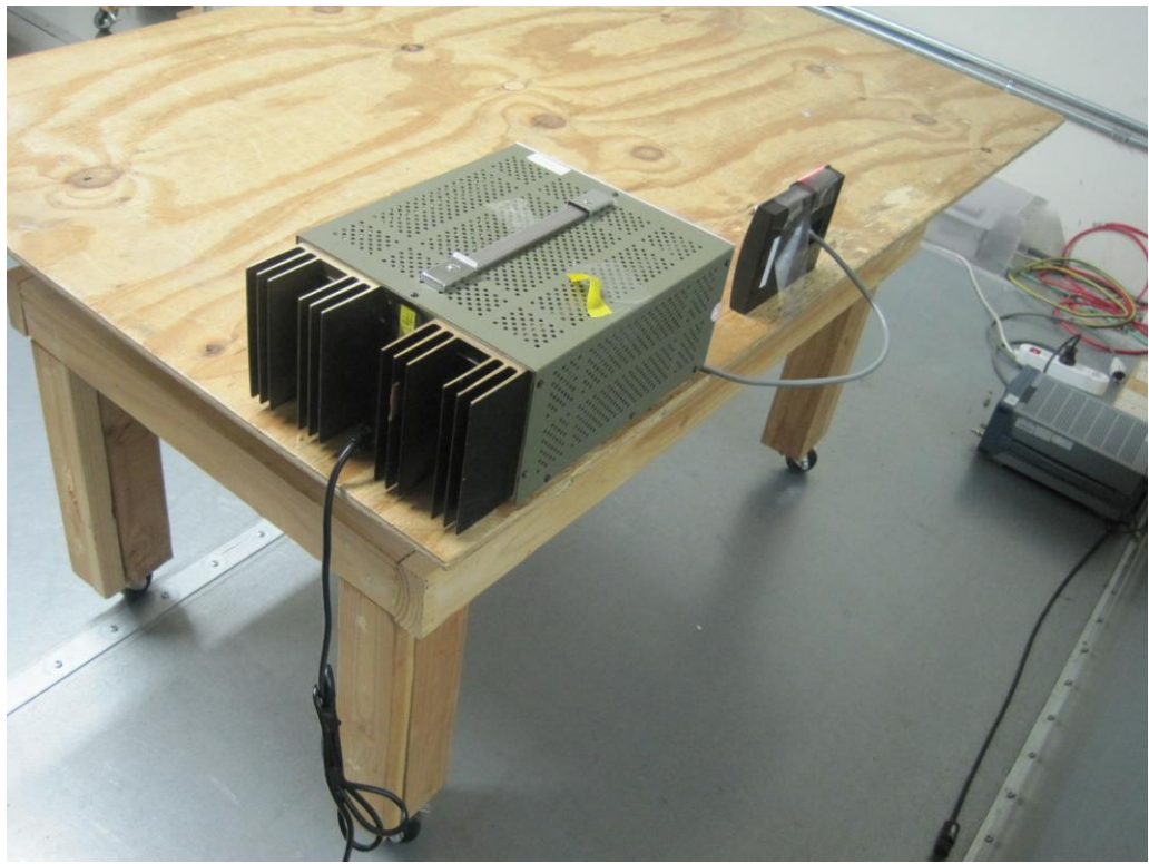
Conducted Emission Test Setup – Rear View ( Pig-Tail Connectors)
