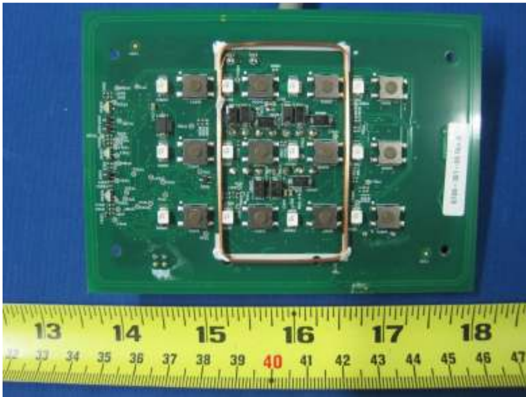
RPKCL40A Pig Tail Back View
