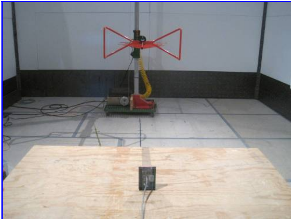
Radiated Emission, Model RPK40D (>30MHz) – Rear View
