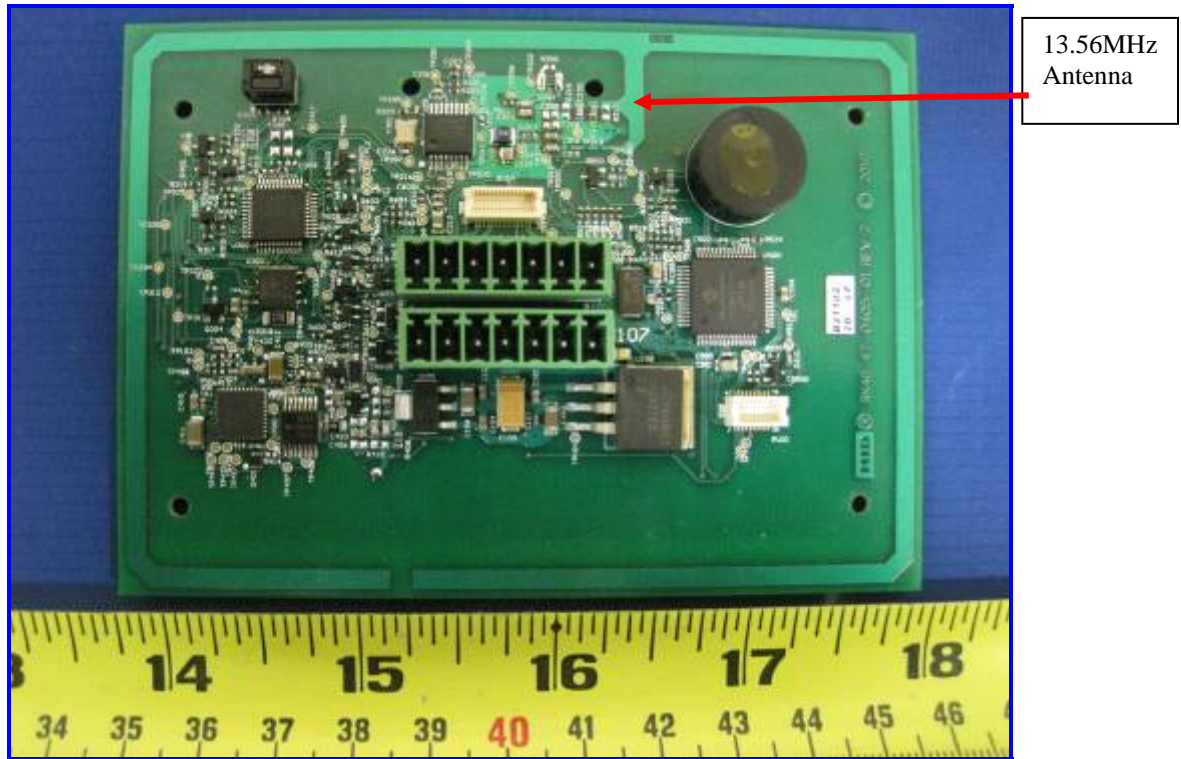
13.56MHz RPK Reader Radio Board – Component View
