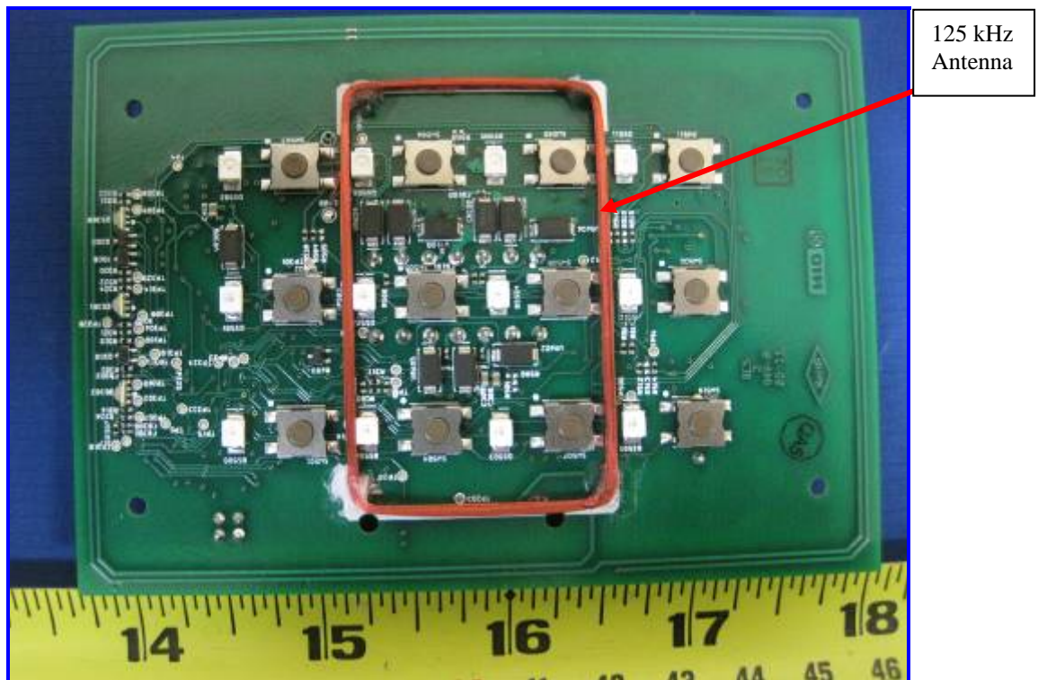
125 kHz RPK Reader Radio Board – Solder/Keypad View
