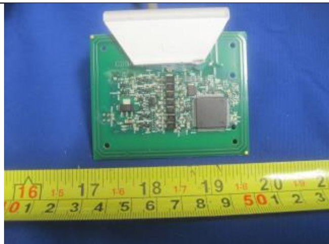
Main PCBA Top View (Pigtail Connector)
