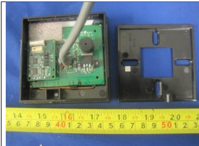
Cover Off View (Pigtail Connector)
