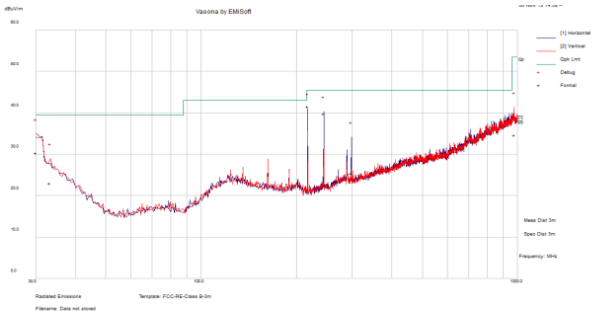
30MHz to 1000MHz at 3m
