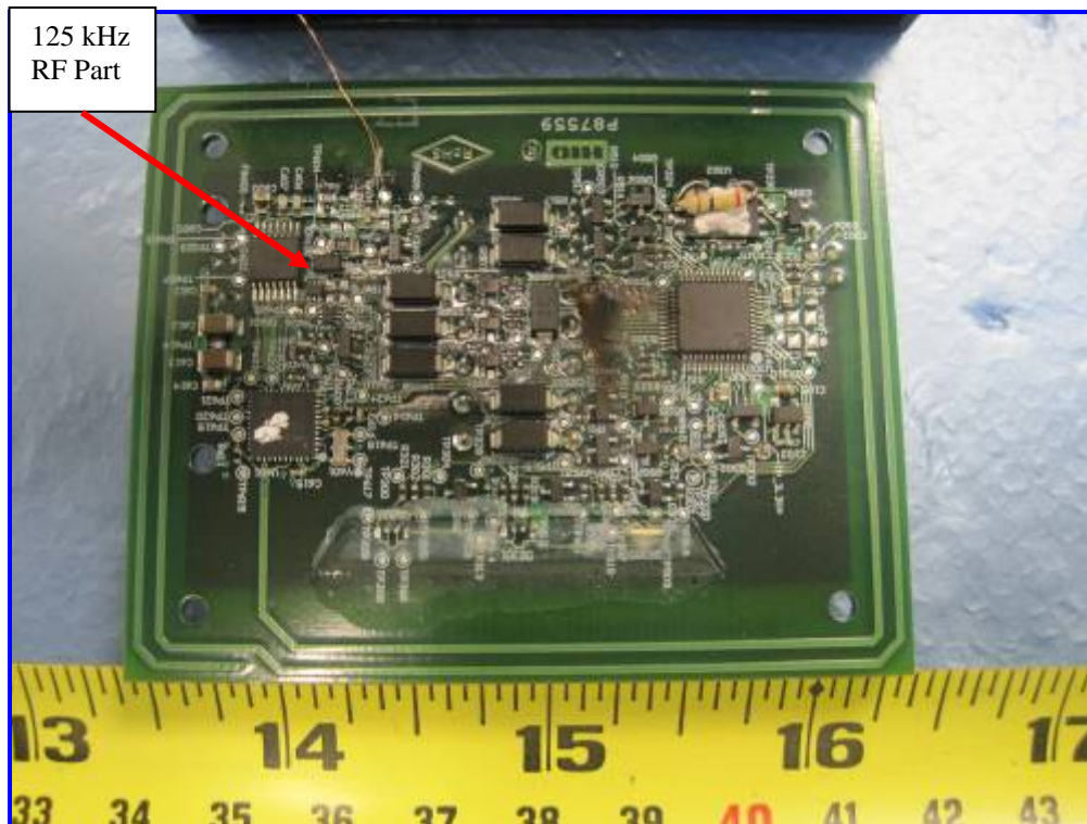
125kHz RP Reader Radio Board View
