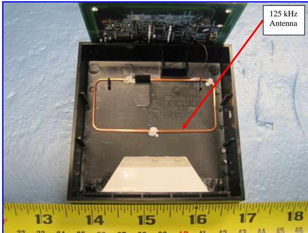
125kHz RP Reader Antenna View
