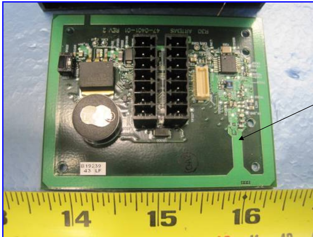
13.56MHz RP Reader Radio Board – Component View
