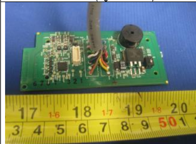
Main PCBA Bottom View (Pigtail Connector)
