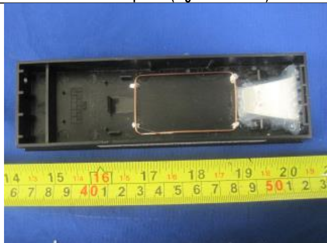
Loop Antenna (Pigtail Connector)
