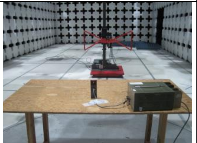
Radiated Emissions (<1GHz) – Rear View (Pigtail Connector)
