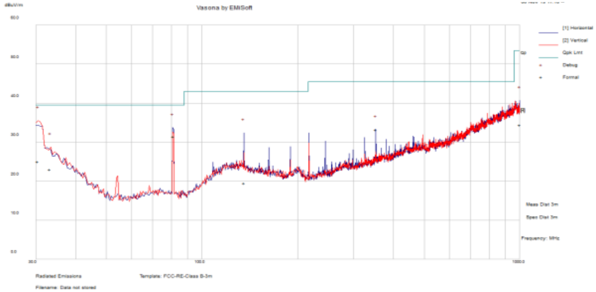
30MHz to 1000MHz at 3m
