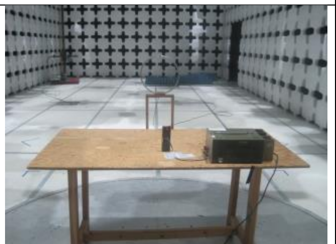
Radiated Emissions (<30MHz) – Rear View (Pigtail Connector)
