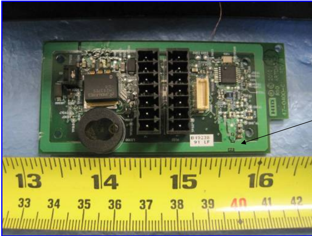
13.56MHz RP Reader Radio Board – Component View
