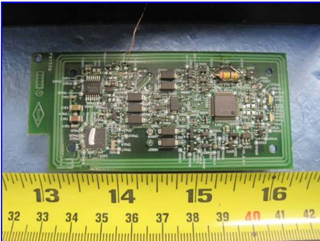
13.56MHz RP Reader Radio Board – Solder View
