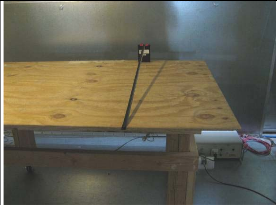
AC Line Conducted Emission Test Setup – Front View 1 (RP40)
