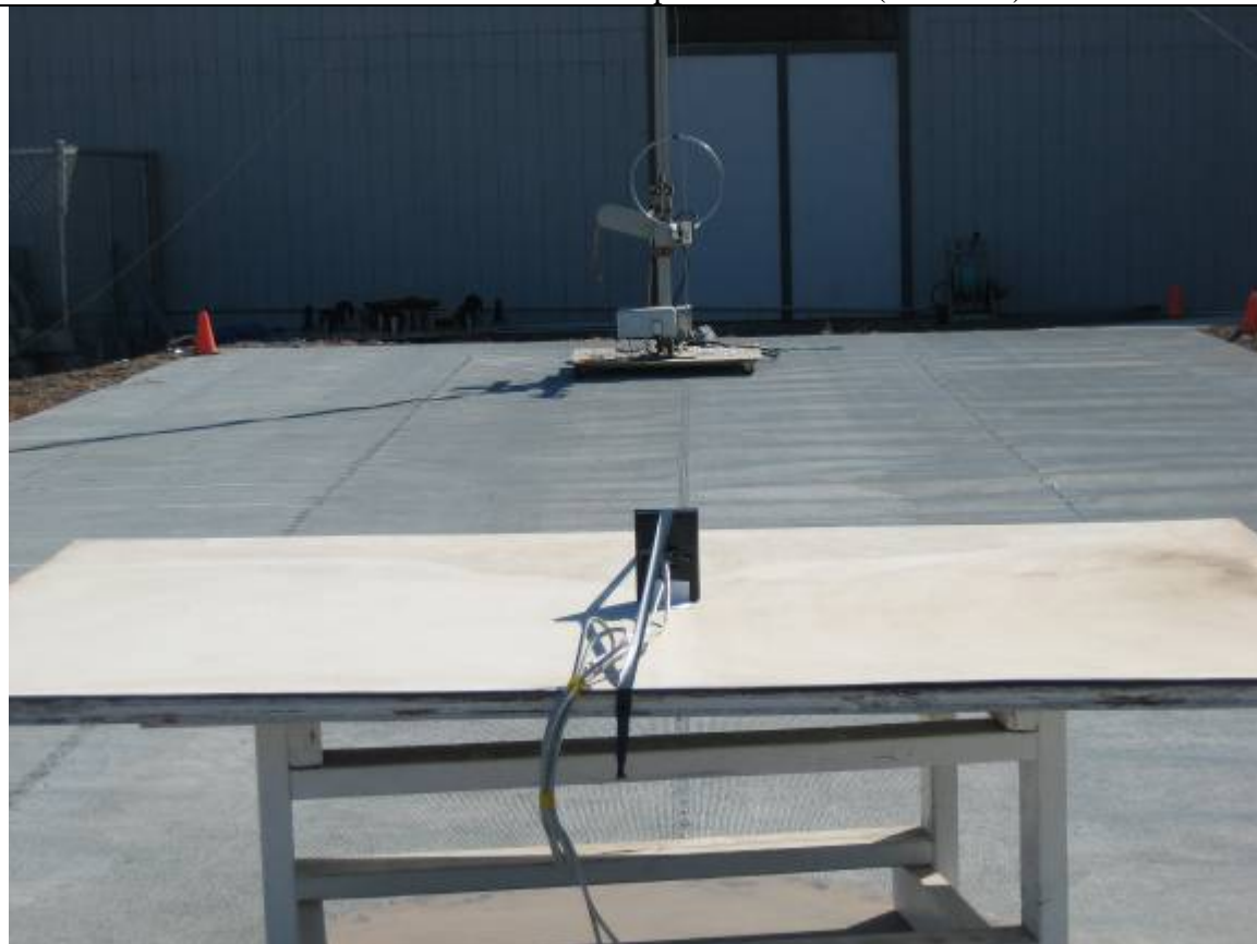
Radiated Emission Test Setup – Rear View (<30MHz)
