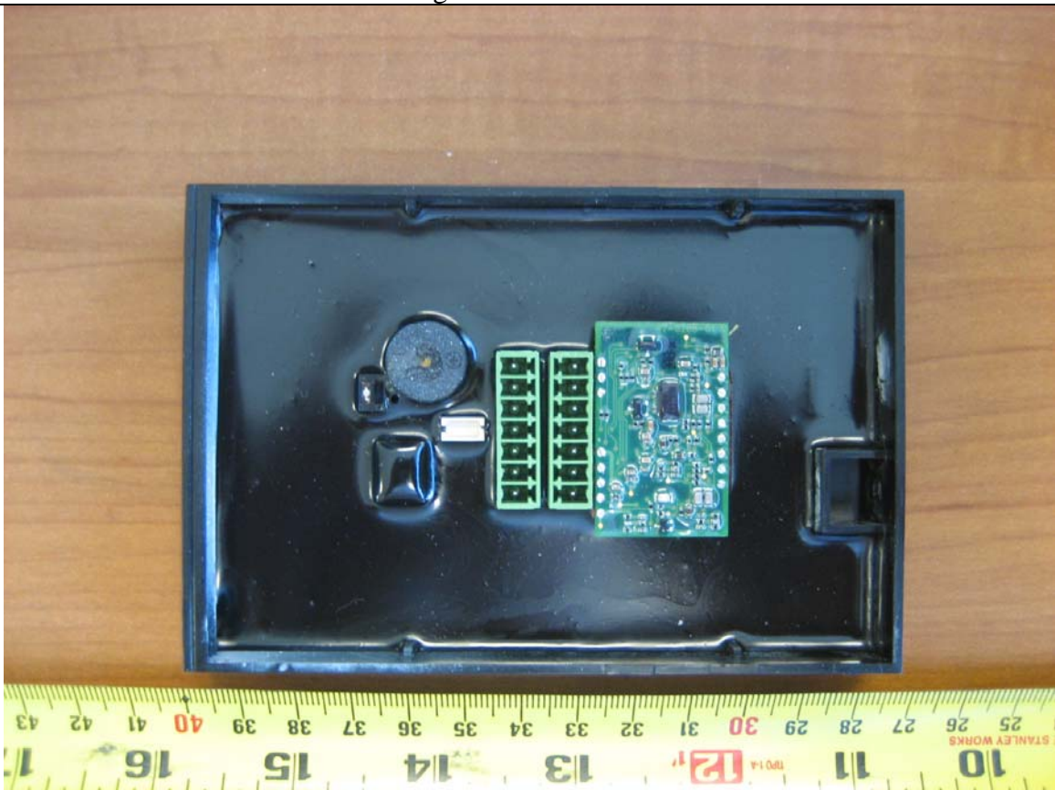
Reader Board with Digital I/O Board in Plastic Housing – Potted
