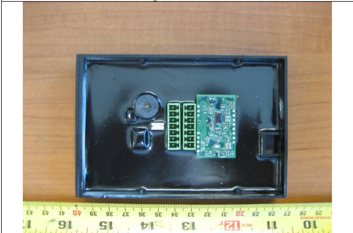
Reader Board with Digital I/O Board in Plastic Housing – Potted
