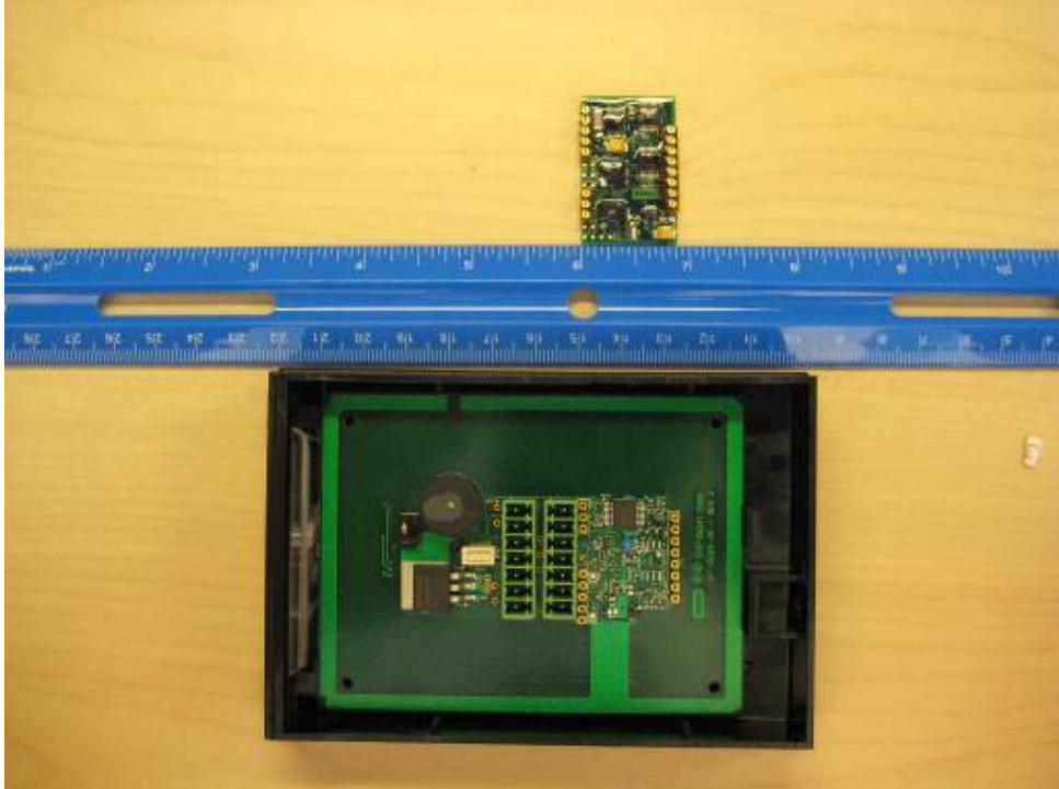
Reader Board in Plastic Housing without Digital I/O Board – Not Potted
