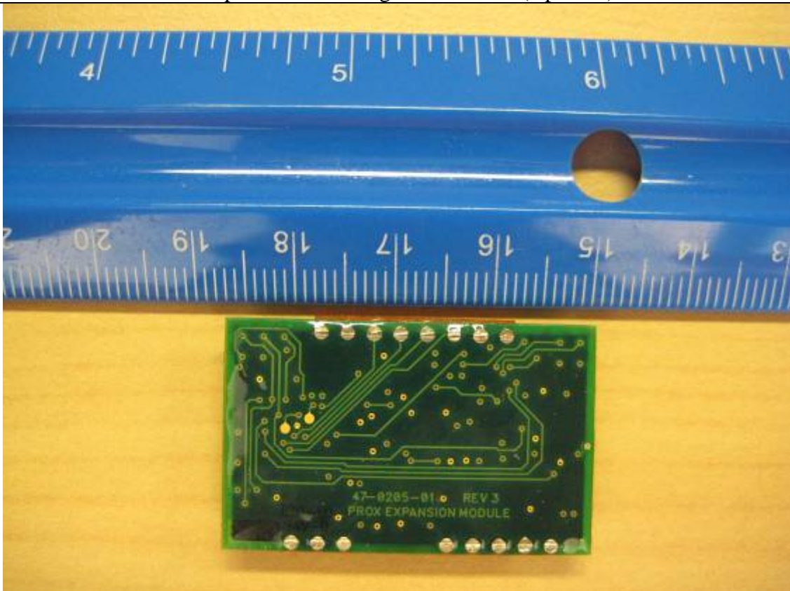
Solder side of Digital I/O Board (Optional)
