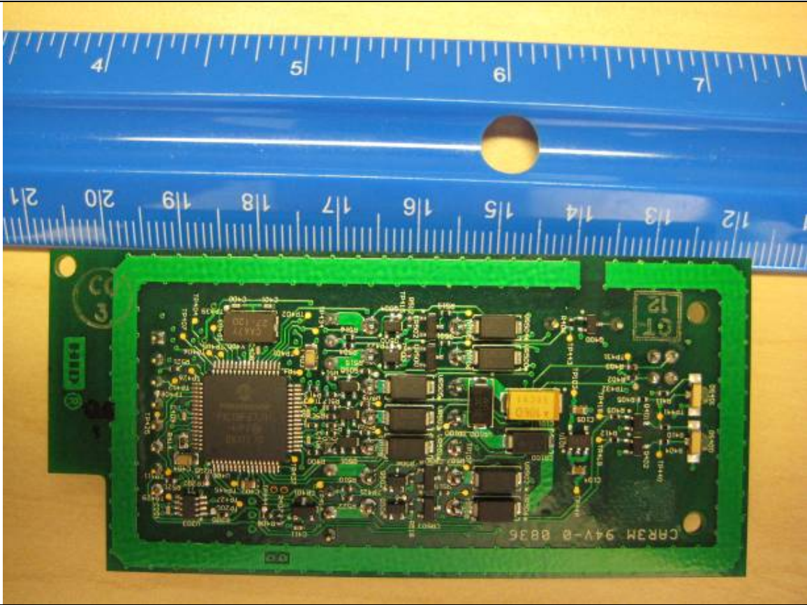
Front side of Reader Board
