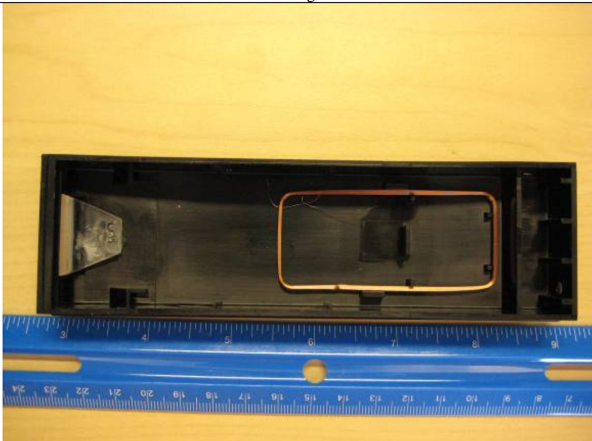
Antenna in Plastic Housing after Reader Board Removed
