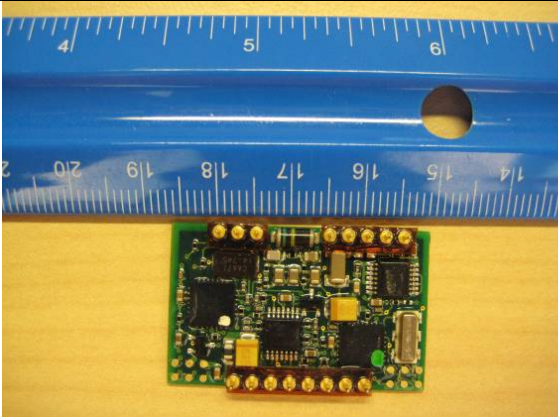
Component side of Digital I/O Board (Optional)
