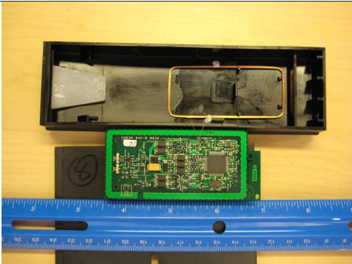
Reader Board in Plastic Housing with Antenna – Not Potted
