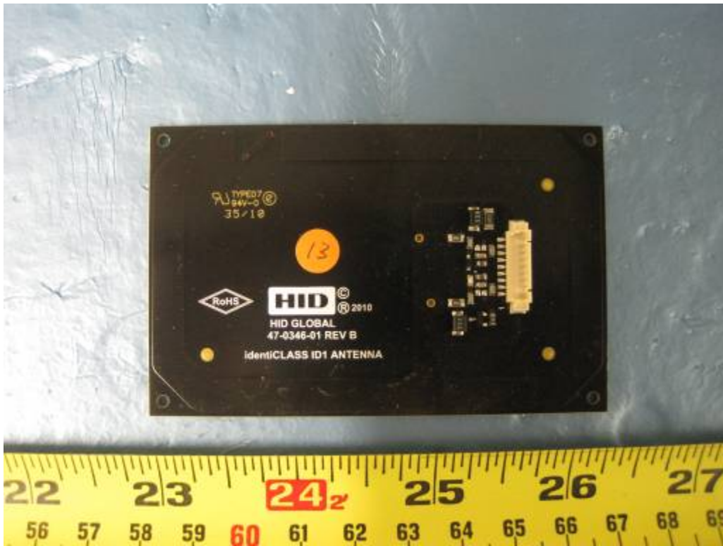
Antenna ID1 Top View
