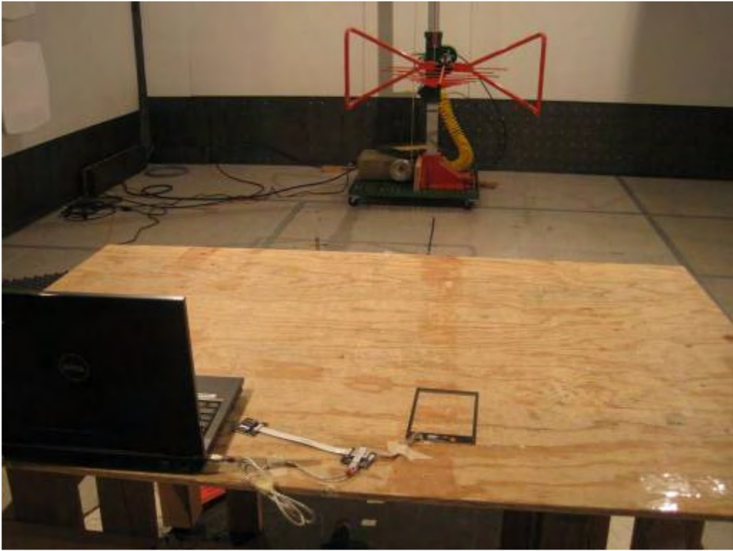
Radiated Emission Test >30MHz (Rear View) --- identiCLASS 3300 + Antenna ID3 + SAM ID0
