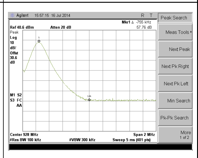
Band Edge-High Channel (Hopping mode)
