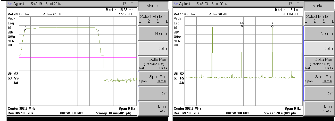
FCC-15.247-DwT-902.75M
