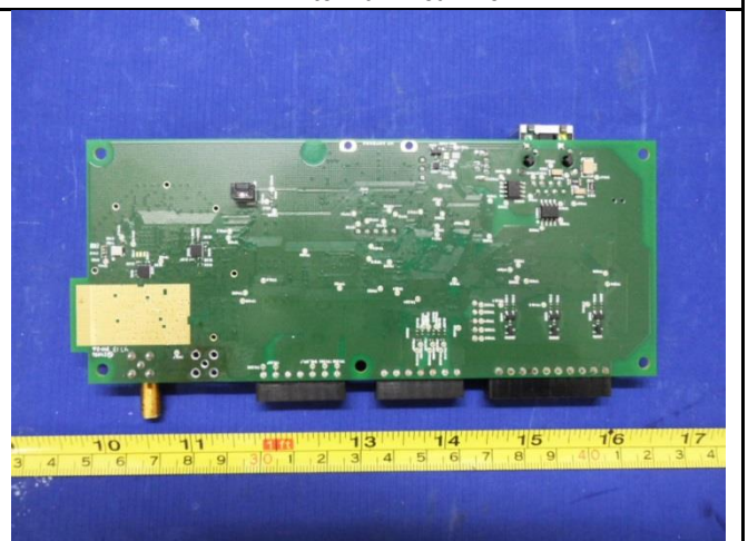
PCB Controller - Rear View
