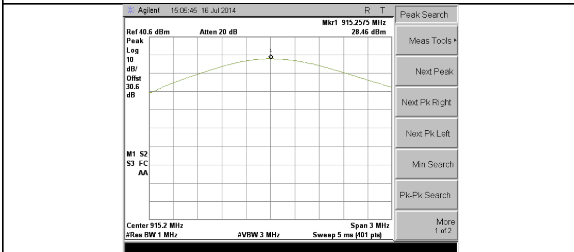
FCC-15.247-PWR-915.25M
