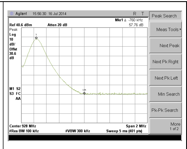
Band Edge-High Channel (Single CH Cont-TX)
