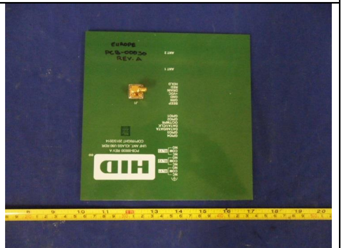
RFID Antenna - Rear View
