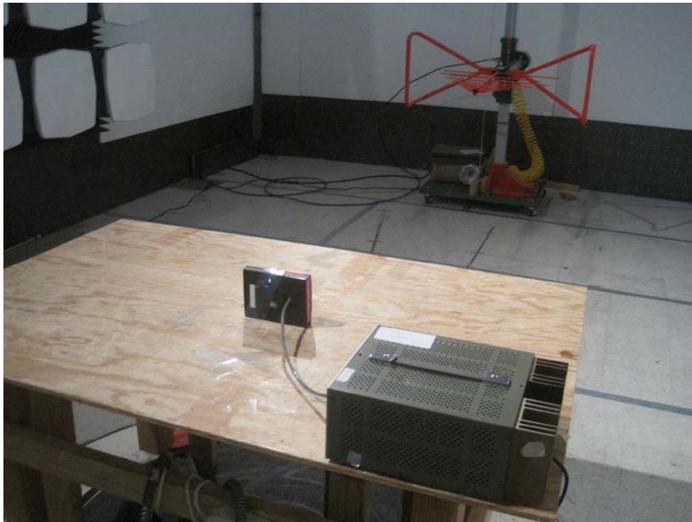
Radiated Emission>30MHz Test Setup – Rear View
