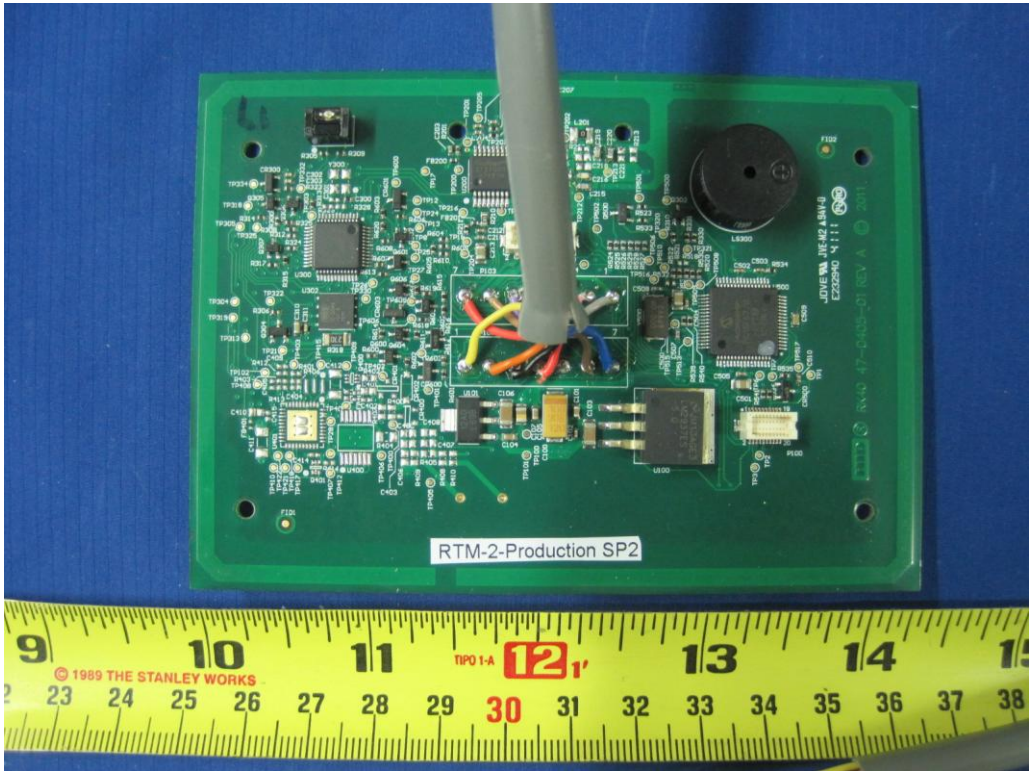
RKCL40A Pig Tail Front View
