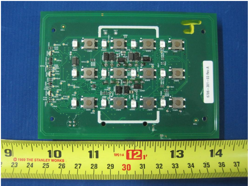
RKCL40A Terminal Back View
