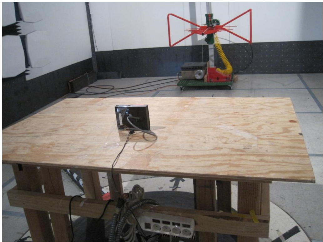
Radiated Emission Test Setup – Rear View ( Pig-Tail Connectors)
