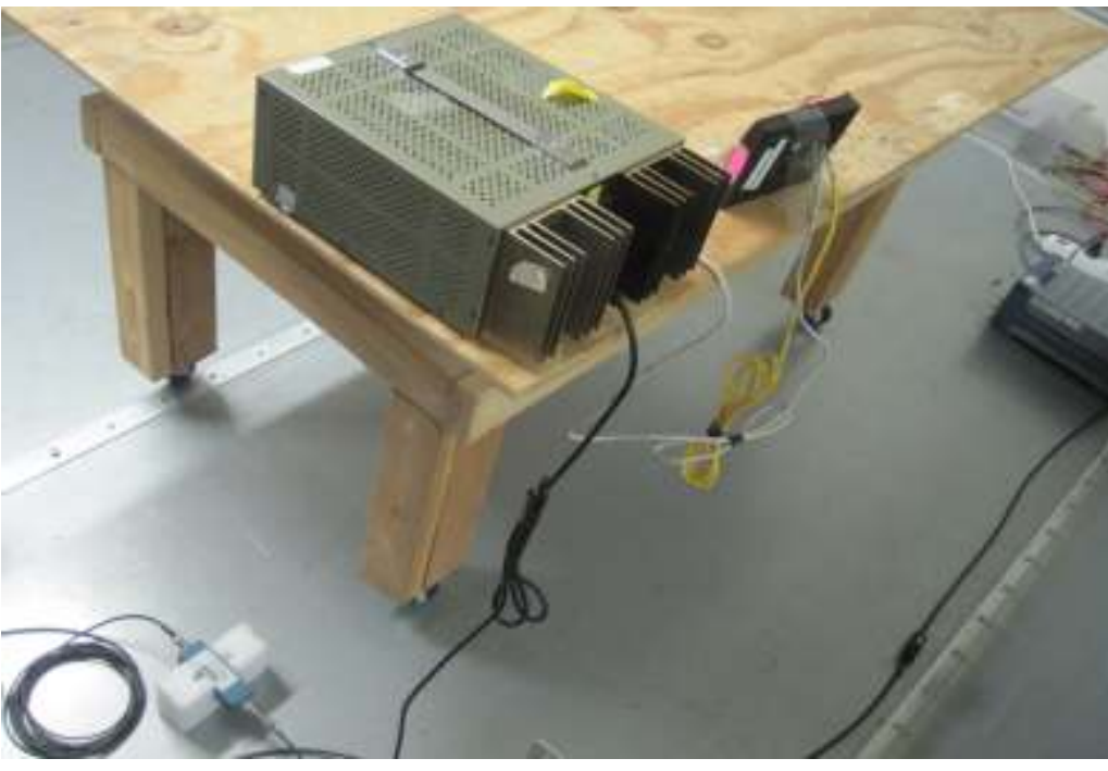
Conducted Emission Test Setup – Rear View (Terminal Connectors)
