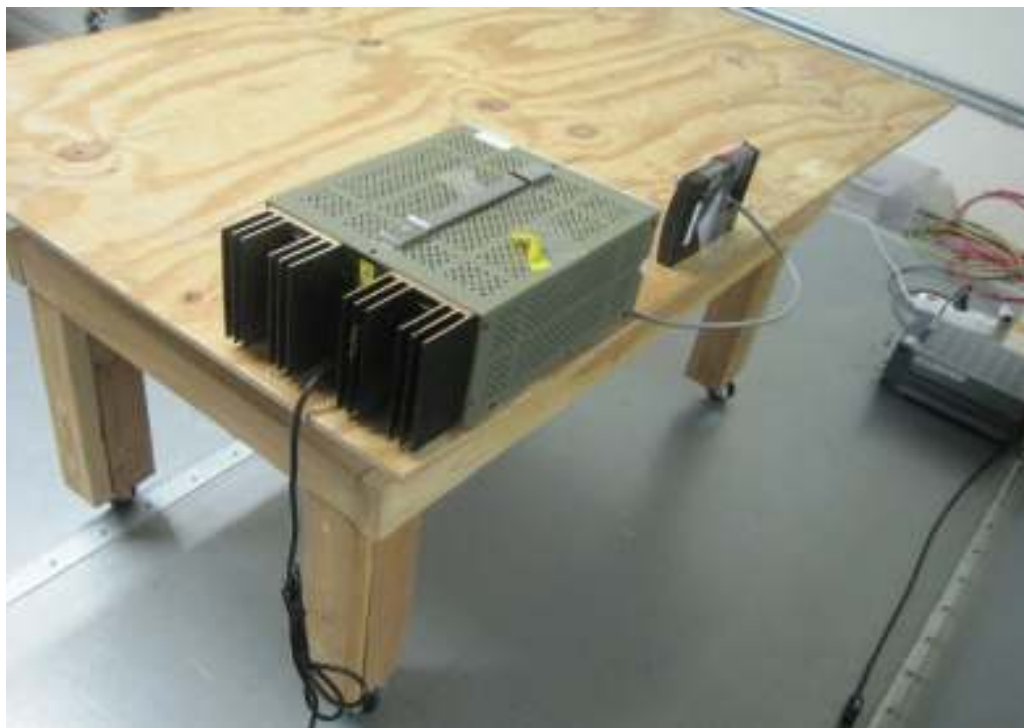
Conducted Emission Test Setup – Rear View ( Pig-Tail Connectors)
