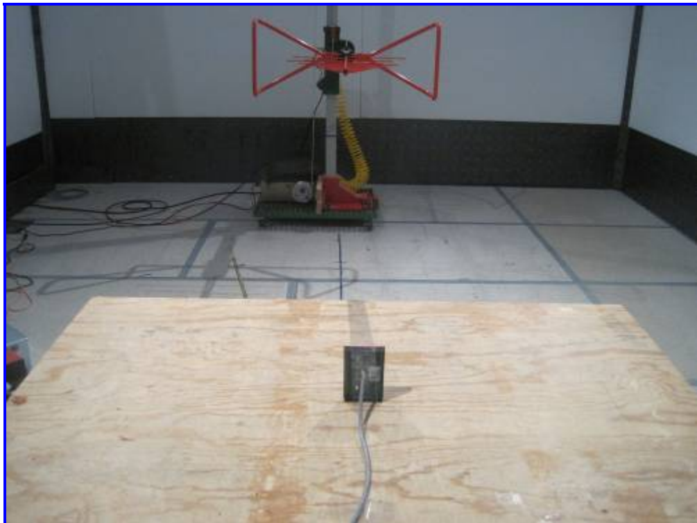
Radiated Emission, Model RK40D (>30MHz) – Rear View
