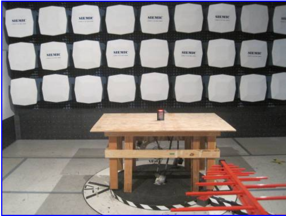
Radiated Emission, Model RK40D (>30MHz) – Front View
