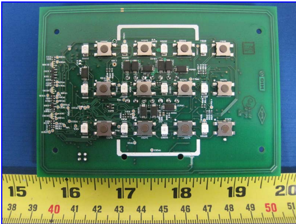
13.56MHz RK Reader Radio Board – Solder/Keypad View
