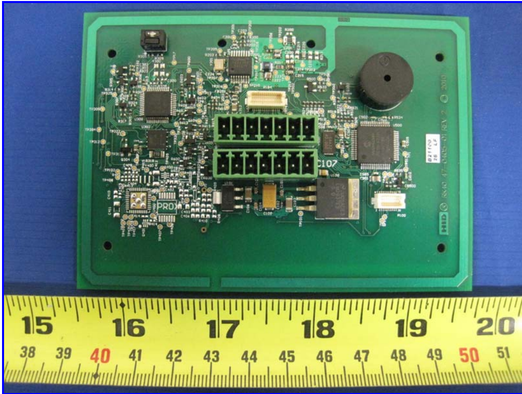
13.56MHz RK Reader Radio Board – Component View
