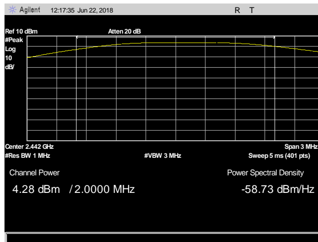
Plot 7. Peak Power Output, 2442
