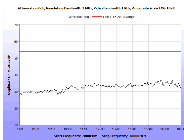
Plot 17. Radiated Emissions, 7 GHz – 18 GHz, Vertical, Average
