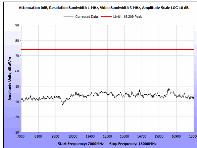
Plot 16. Radiated Emissions, 7 GHz – 18 GHz, Horizontal, Peak
