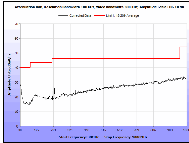
Plot 9. Radiated Emissions, 30 MHz – 1 GHz, Horizontal
