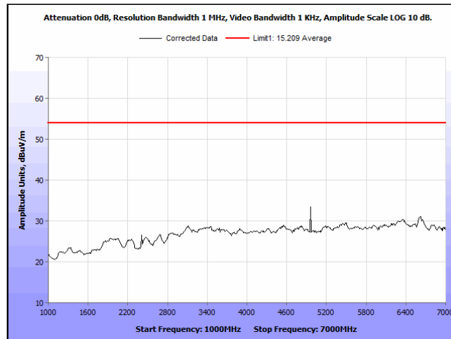
Plot 13. Radiated Emissions, 1 GHz – 7 GHz, Vertical, Average
