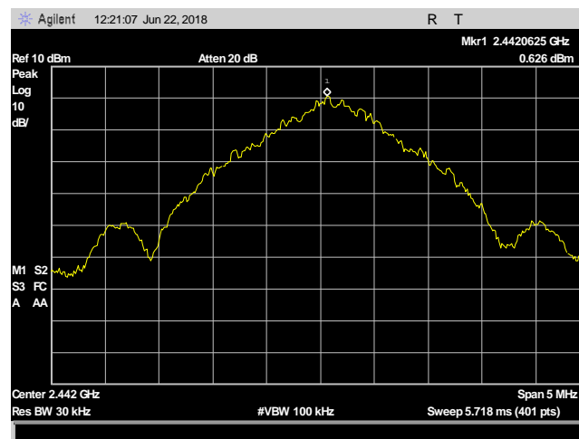
Plot 36. Power Density, 2442
