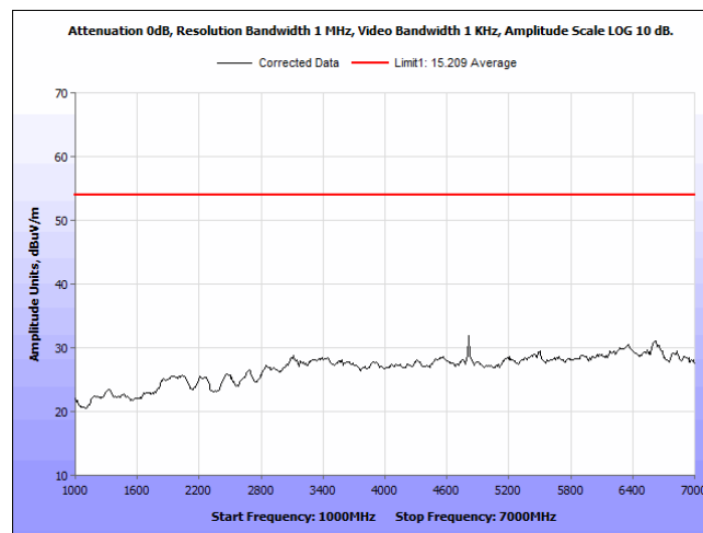
Plot 11. Radiated Emissions, 1 GHz – 7 GHz, Horizontal, Average
