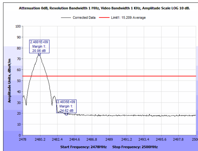
Plot 23. Radiated Restricted Bandedge, 2480, Horizontal, Average
