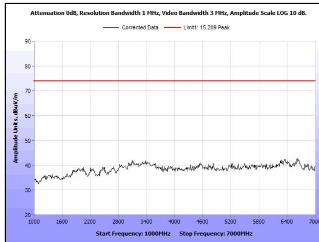
Plot 12. Radiated Emissions, 1 GHz – 7 GHz, Horizontal, Peak
