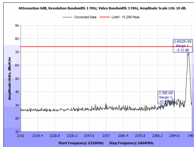
Plot 22. Radiated Restricted Bandedge, 2402, Vertical, Peak
