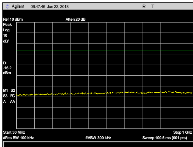
Plot 32. Conducted Spurious Emissions, 2480, 30 MHz – 1 GHz
