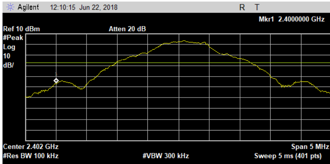
Plot 33. Conducted Spurious Emissions, 2402, Bandedge
