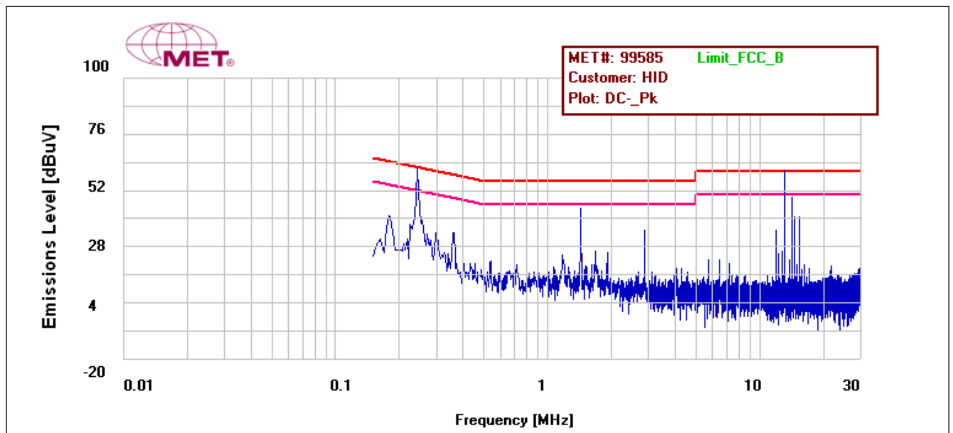
Plot 2. Conducted Emissions, 15.207(a), DC-
