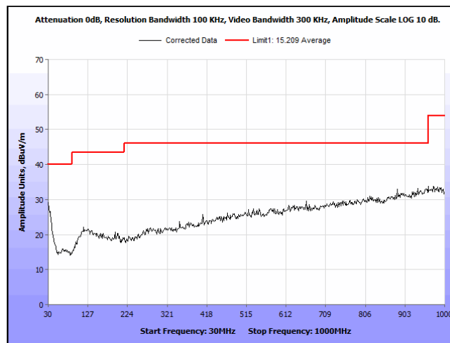
Plot 10. Radiated Emissions, 30 MHz – 1 GHz, Vertical
