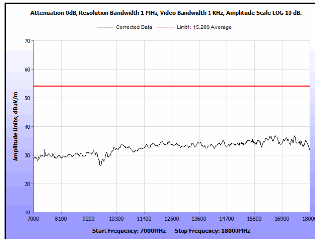
Plot 15. Radiated Emissions, 7 GHz – 18 GHz, Horizontal, Average
