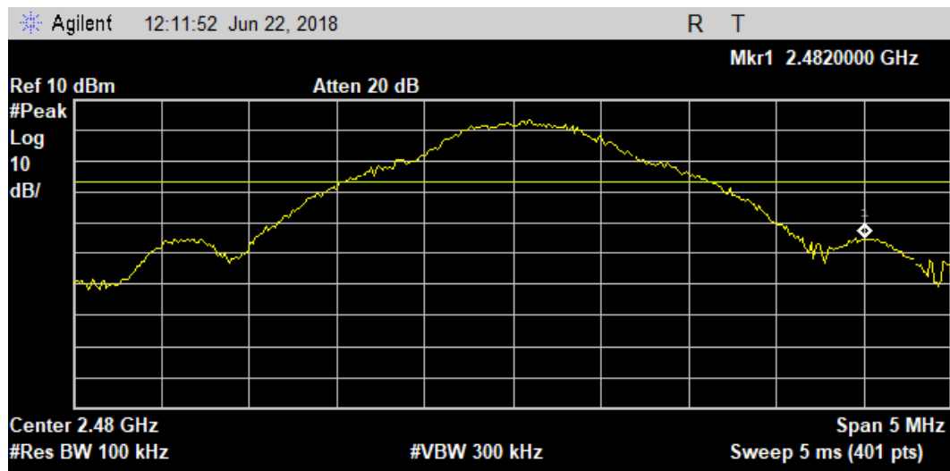
Plot 34. Conducted Spurious Emissions, 2480, Bandedge
