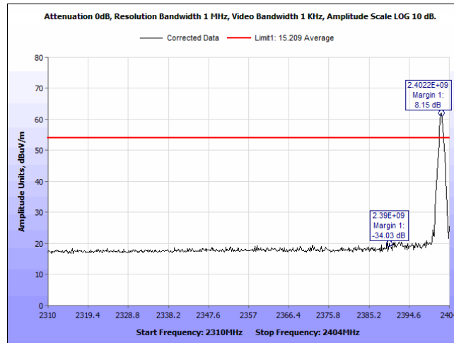
Plot 21. Radiated Restricted Bandedge, 2402, Vertical, Average
