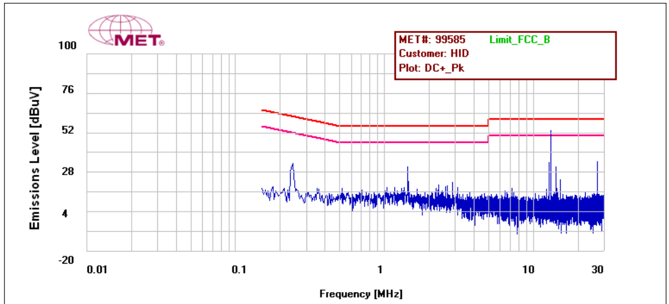
Plot 1. Conducted Emissions, 15.207(a), DC+
