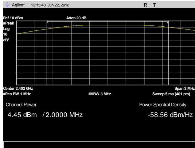
Plot 6. Peak Power Output, 2402
