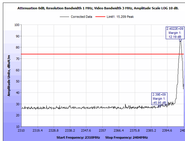
Plot 20. Radiated Restricted Bandedge, 2402, Horizontal, Peak
