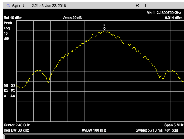
Plot 37. Power Density, 2480
