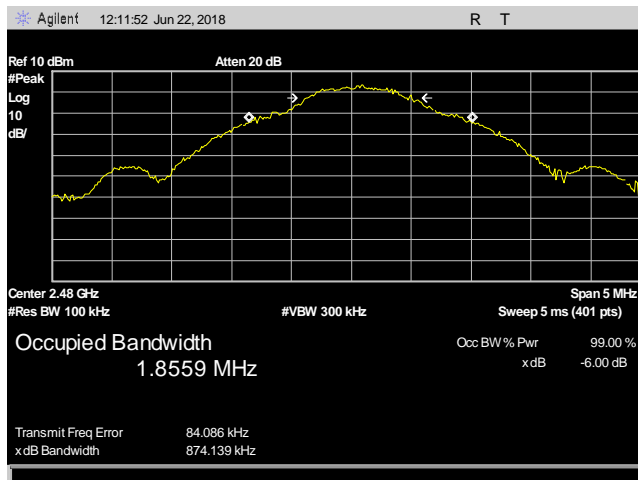
Plot 5. 6 dB Occupied Bandwidth, 2480
