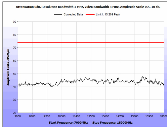
Plot 18. Radiated Emissions, 7 GHz – 18 GHz, Vertical, Peak
