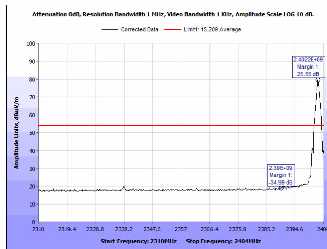
Plot 19. Radiated Restricted Bandedge, 2402, Horizontal, Average
