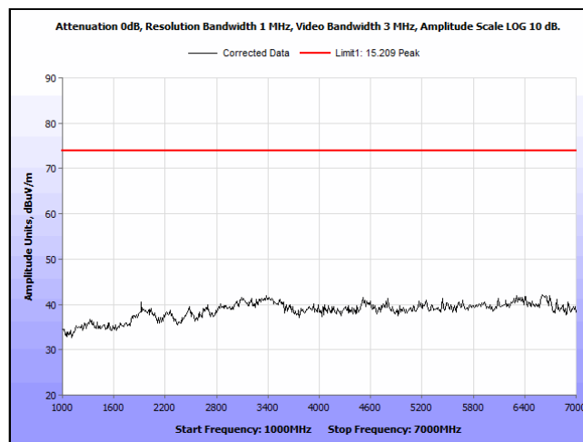
Plot 14. Radiated Emissions, 1 GHz – 7 GHz, Vertical, Peak
