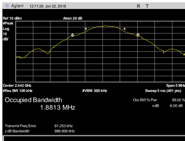
Plot 4. 6 dB Occupied Bandwidth, 2442
