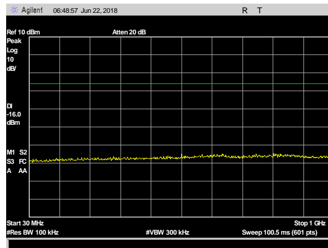
Plot 28. Conducted Spurious Emissions, 2402, 30 MHz – 1 GHz
