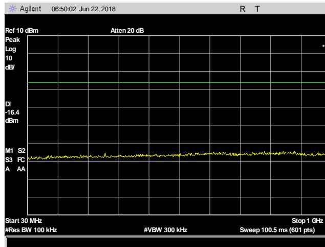
Plot 30. Conducted Spurious Emissions, 2442, 30 MHz – 1 GHz
