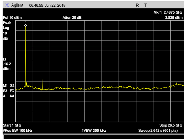
Plot 31. Conducted Spurious Emissions, 2480, 1 – 26.5 GHz
