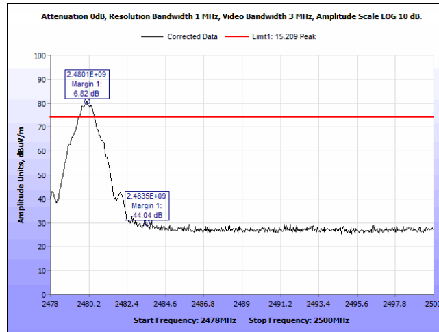
Plot 24. Radiated Restricted Bandedge, 2480, Horizontal, Peak
