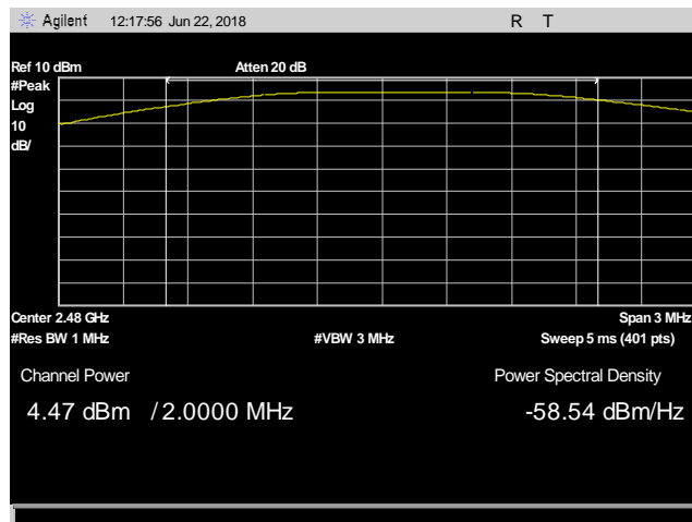
Plot 8. Peak Power Output, 2480
