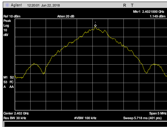
Plot 35. Power Density, 2402
