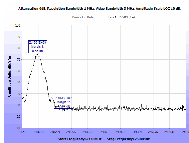
Plot 26. Radiated Restricted Bandedge, 2480, Vertical, Peak
