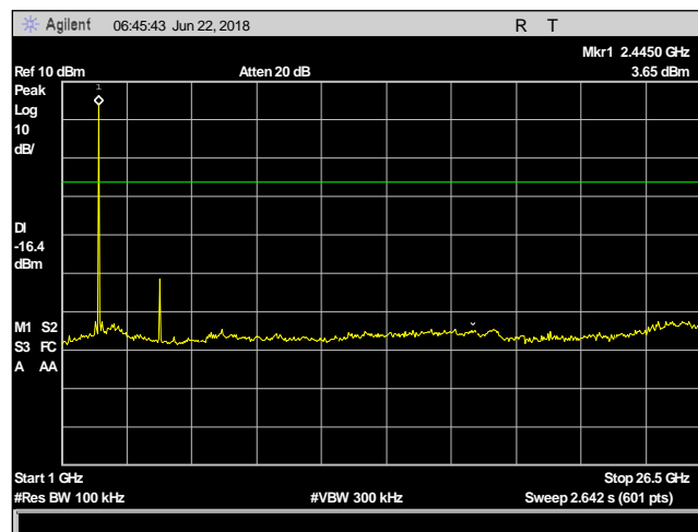
Plot 29. Conducted Spurious Emissions, 2442, 1 – 26.5 GHz
