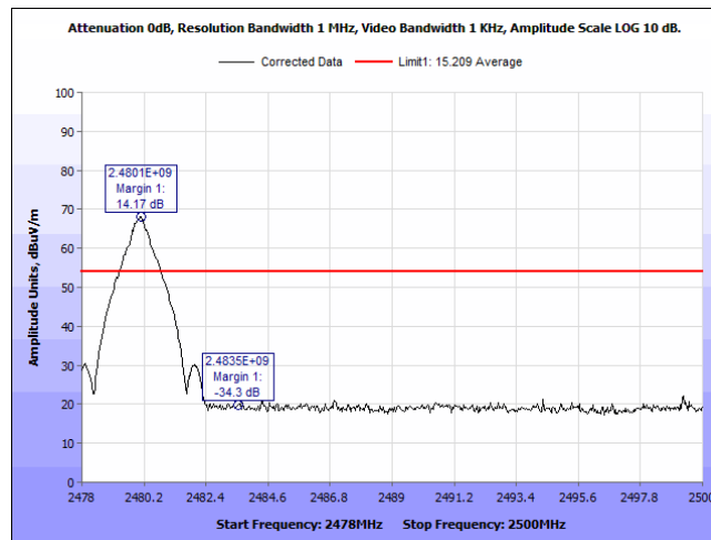
Plot 25. Radiated Restricted Bandedge, 2480, Vertical, Average
