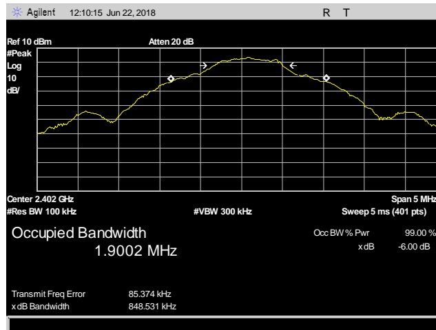
Plot 3. 6 dB Occupied Bandwidth, 2402
