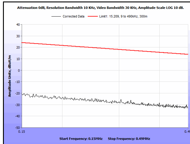
Plot 9. Spurious Emissions, Outside the Band 13.110 - 14.010 MHz, 150 – 490 kHz, 90 degrees
