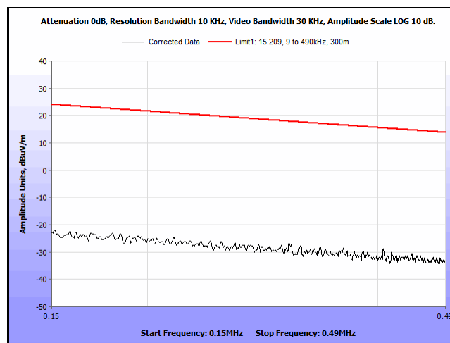
Plot 8. Spurious Emissions, Outside the Band 13.110 - 14.010 MHz, 150 – 490 kHz, 0 degrees
