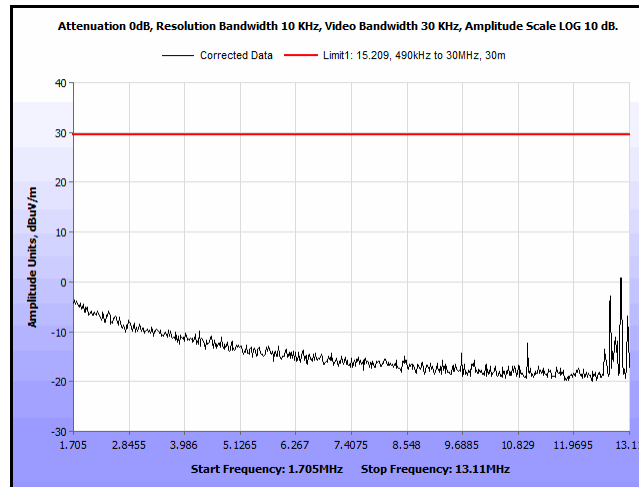
Plot 12. Spurious Emissions, Outside the Band 13.110 - 14.010 MHz, 1.705 – 13.11 MHz, 0 degrees
