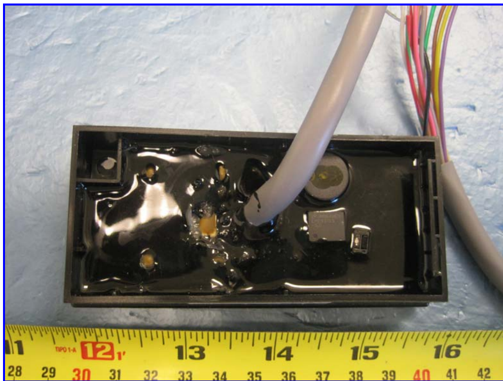
Pig Tail
