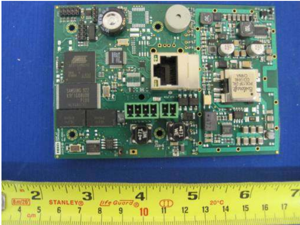
Radio Board A – Bottom
