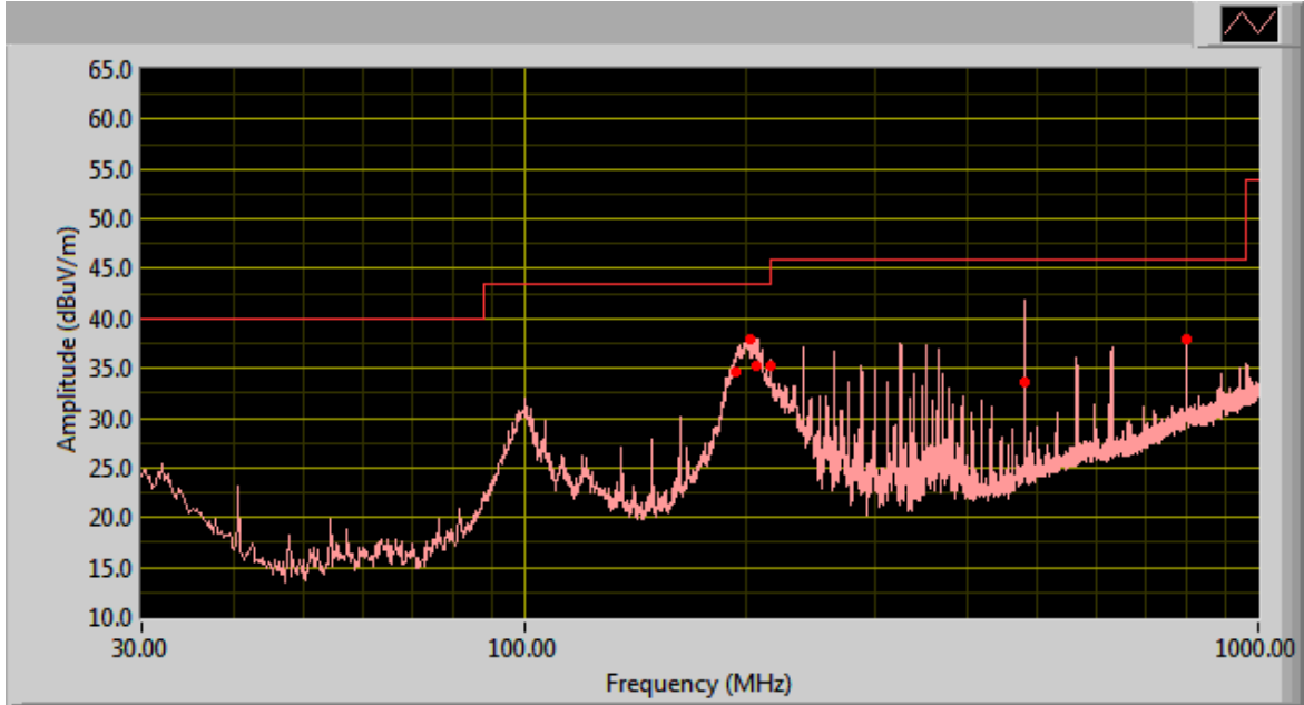
30MHz ~1000MHz Result @ 3m
