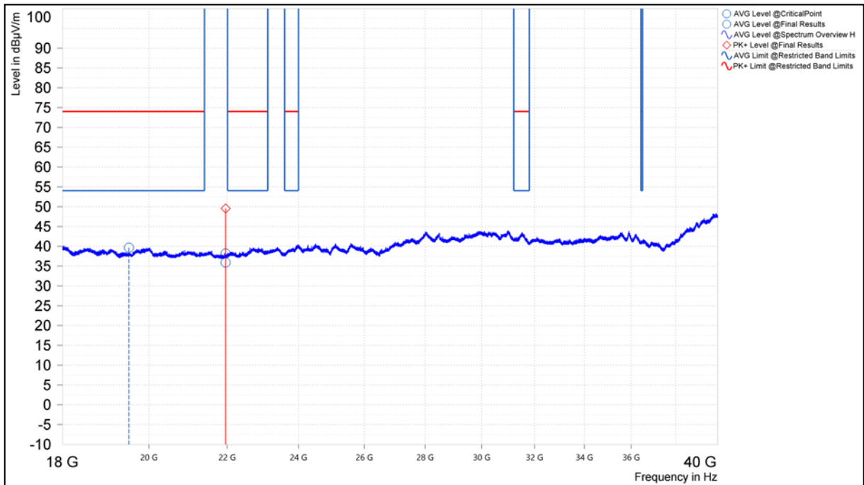
Figure 34. Worst Case Cabinet Radiation, 18GHz – 40GHz, Horizontal Polarity
