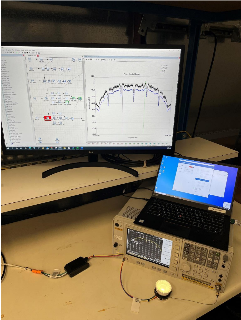
Conducted Antenna Port Testing
