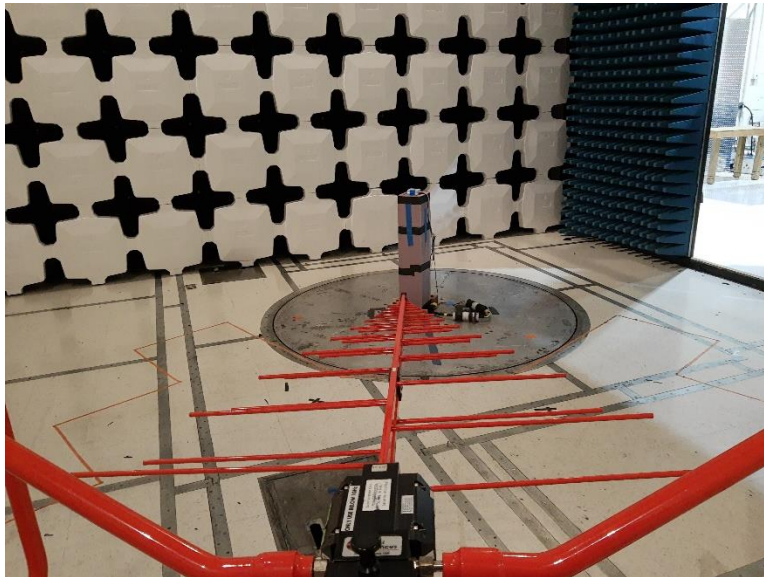
Figure 4: RE Setup [30MHz - 1GHz]
