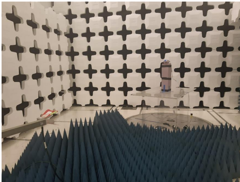
Figure 6: RE Setup [1GHz - 5GHz]
