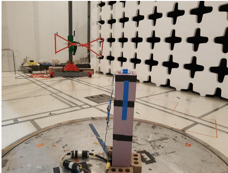
Figure 3: RE Setup [30MHz - 1GHz, Rear]
