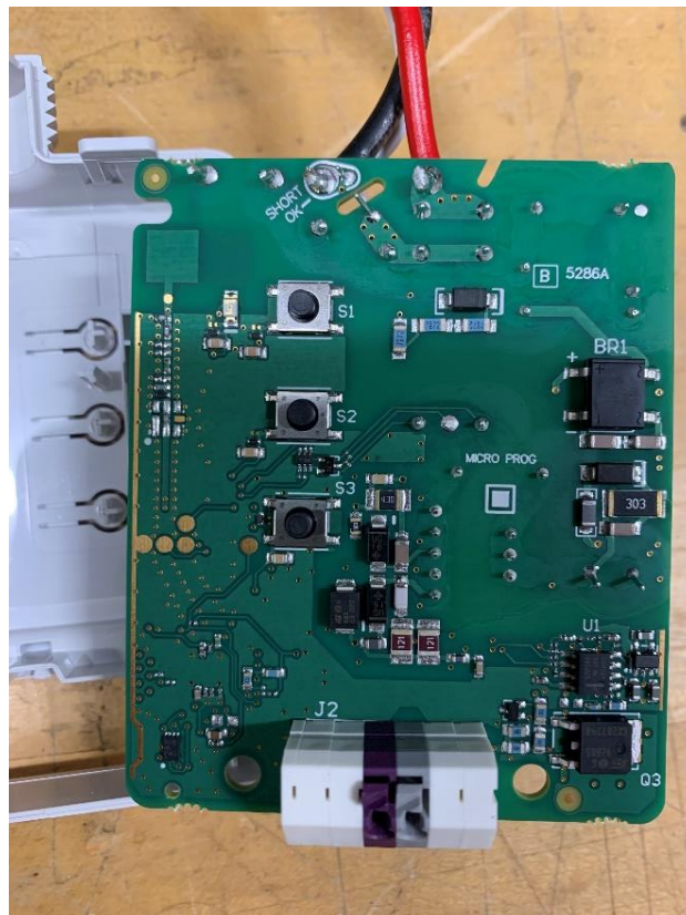
PWB Front
