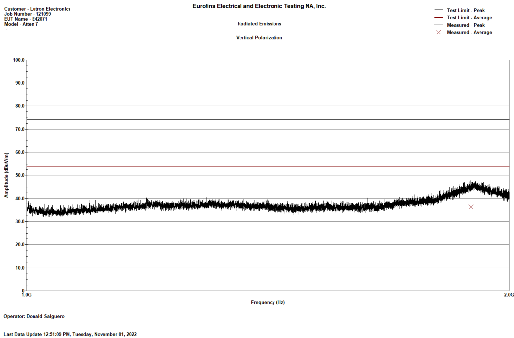
Figure 9. FCC-ICES RE 1-2 GHz Vertical Polarization
