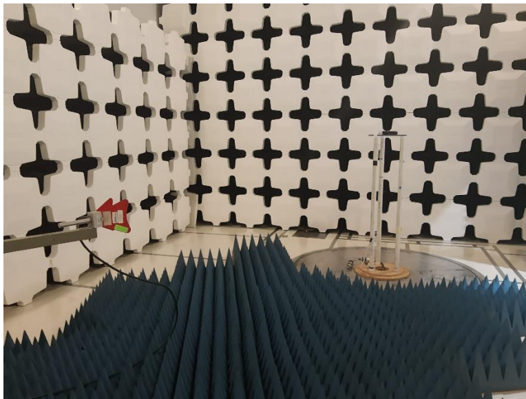
Figure 2. Radiated Emissions - Test Setup, 1-5GHz
