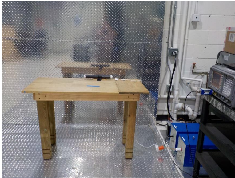
Figure 1. 121493 CEV AC_DC setup
