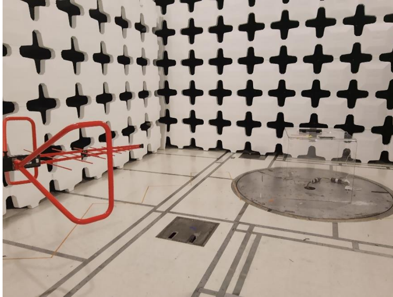
Figure 3. Radiated Emissions - Test Setup, 30-1000MHz
