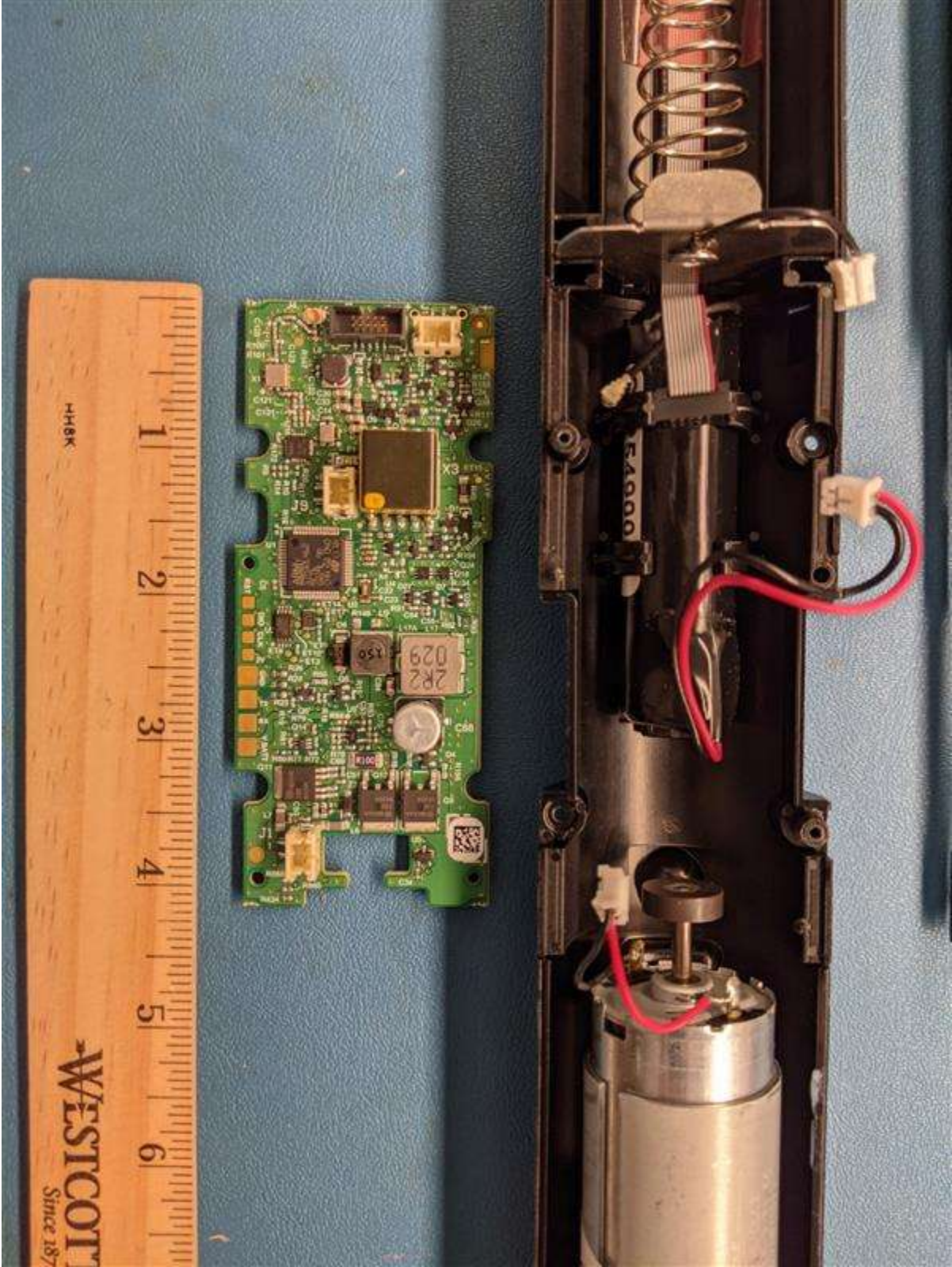
Lutron Model QSFC-EDU-BP-C Chassis with Board
