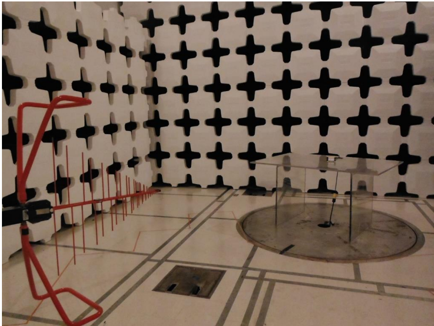
Figure 2: Radiated Spurious Emission Test Setup 30MHz-1GHz
