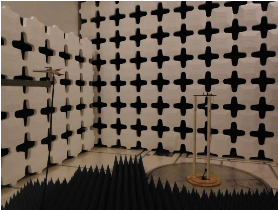
Figure 4: Radiated Spurious Emission Test Setup 18GHz-25GHz
