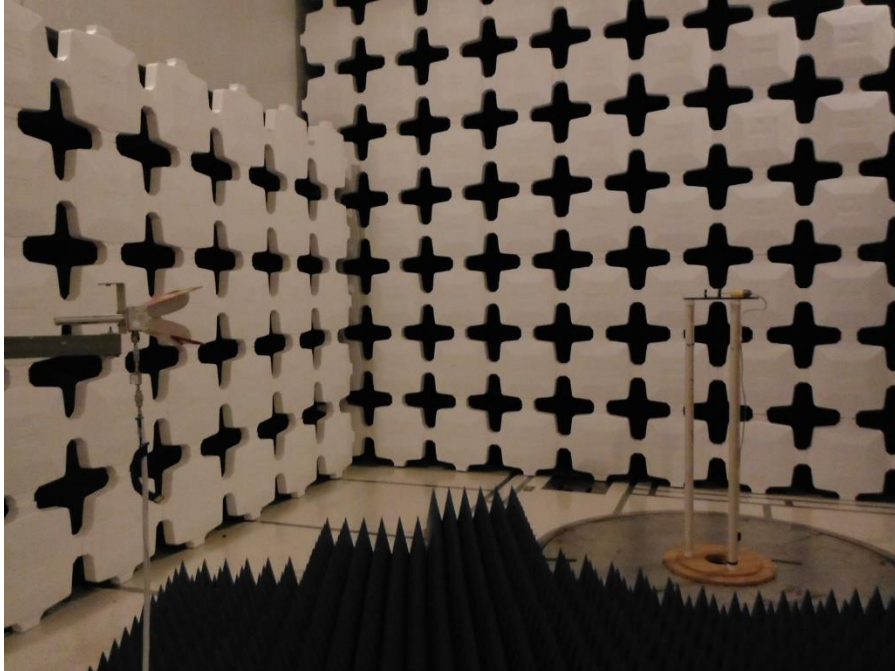
Figure 3: Radiated Spurious Emission Test Setup 1GHz-18GHz
