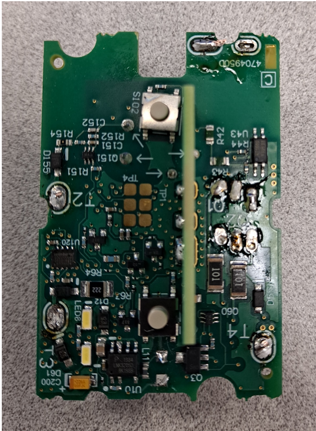
PCB- Top View, SCRs Removed
