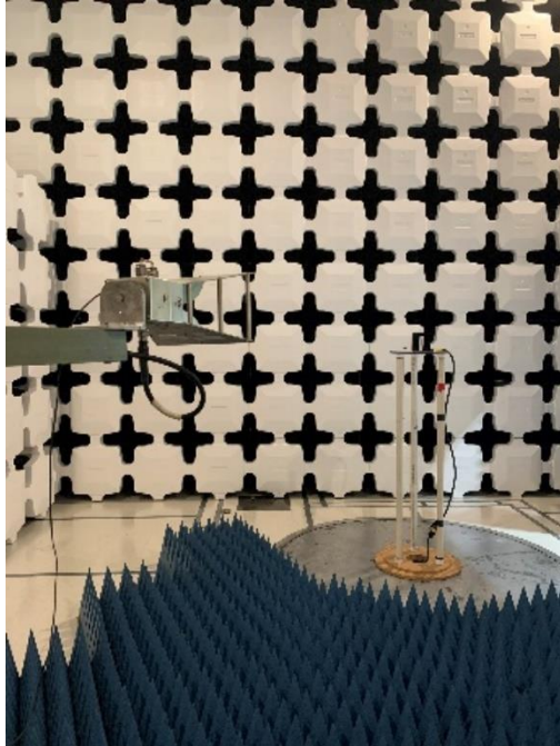
Figure 3: Cabinet Radiated emission setup 1-18GHz
