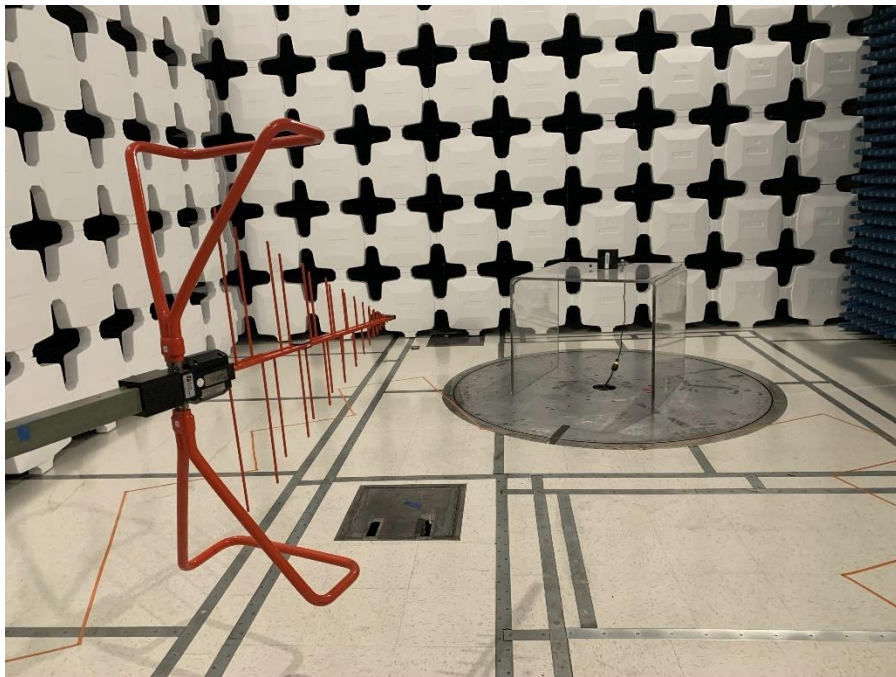
Figure 2: Cabinet Radiated emission setup 30MHz-1GHz
