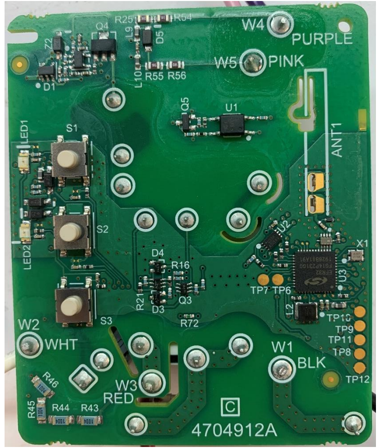
Top of Power Board without Antenna Board
