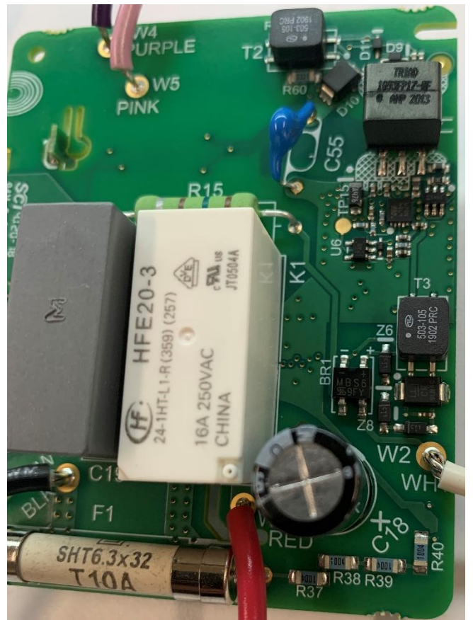
Alternate View of Bottom of Board
