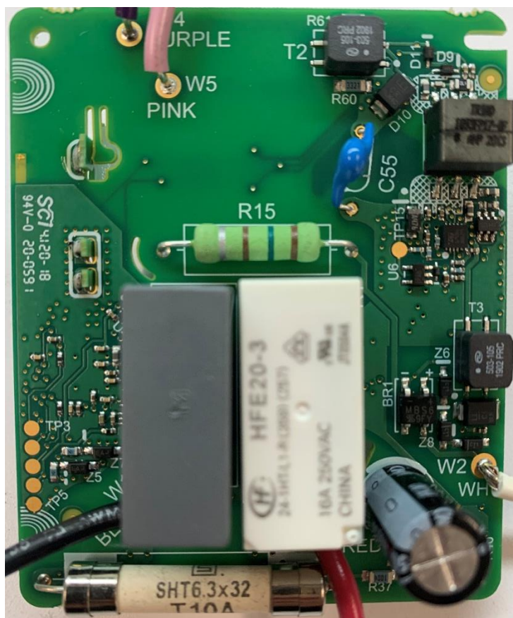
Bottom of Power Board
