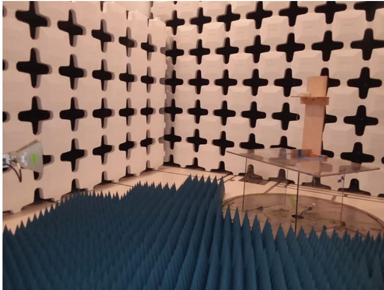
Figure 3: Field Strength of Fundamental and Harmonics, Radiated Emissions, Radiated Emissions, 1GHz – 5GHz, Test Setup
