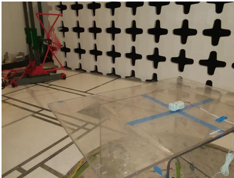
Figure 2: Field Strength of Fundamental and Harmonics, Radiated Emissions, Radiated Emissions, 30MHz – 1GHz, Test Setup
