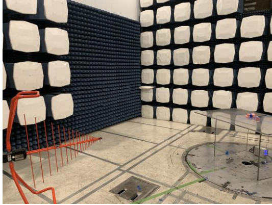
Figure 4: Radiated Emissions, Test Setup, Below 1 GHz Antenna 2
