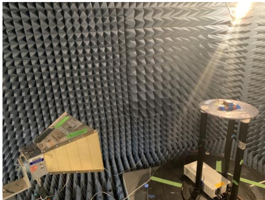
Figure 3: Radiated Emissions, Test Setup, Above 1 GHz Antenna 1
