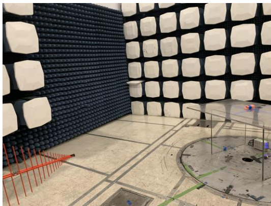
Figure 2: Radiated Emissions, Test Setup, Below 1 GHz Antenna 1
