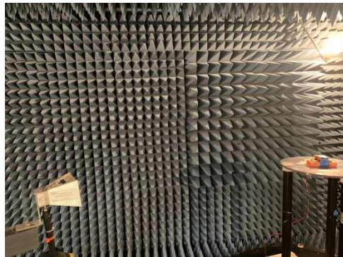
Figure 6: Radiated Emissions, Test Setup, 18 -25 GHz Antenna 1
