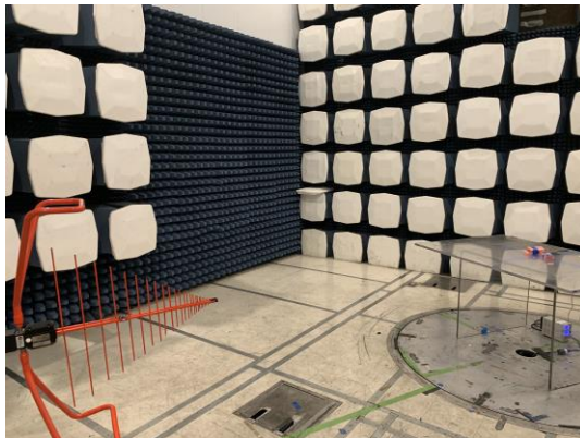
Figure 3: Radiated Emissions, Test Setup, Below 1 GHz Antenna 2
