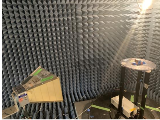
Figure 4: Radiated Emissions, Test Setup, Above 1 GHz Antenna 1
