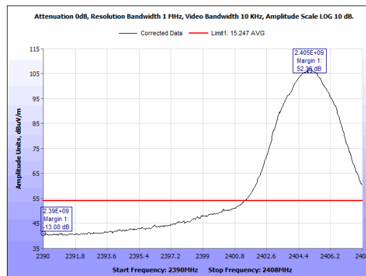
Figure 44: Radiated Emissions, ZigBee Low Channel Band Edge, Average, Antenna 2
