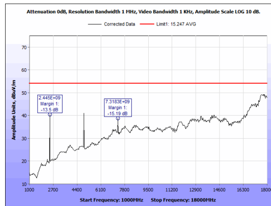
Figure 33: Radiated Emissions, ZigBee, 1GHz - 18GHz, Average, Mid Channel, Antenna 2
