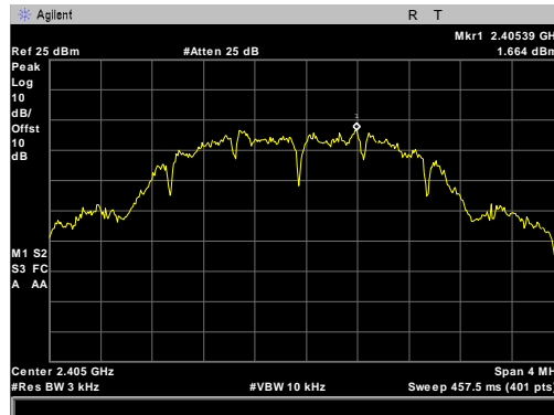
Figure 64: Peak Power Spectral Density, ZigBee, Low Channel,
