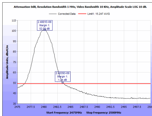
Figure 50: Radiated Emissions, ZigBee High Channel Band Edge, Average, Antenna 2
