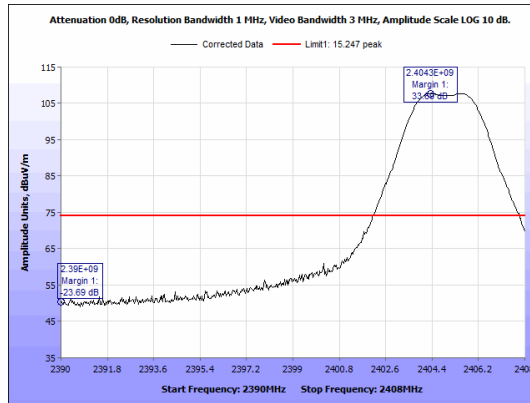
Figure 45: Radiated Emissions, ZigBee Low Channel Band Edge, Peak, Antenna 2
