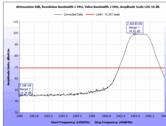
Figure 43: Radiated Emissions, ZigBee Low Channel Band Edge, Peak, Antenna 1
