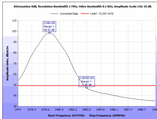
Figure 47: Radiated Emissions, ZigBee High Channel Band Edge, Average, 100Hz Antenna 1
