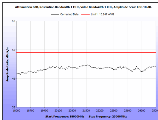
Figure 19: Radiated Emissions, ZigBee, 18GHz - 25GHz, Average, Mid Channel, Antenna 1
