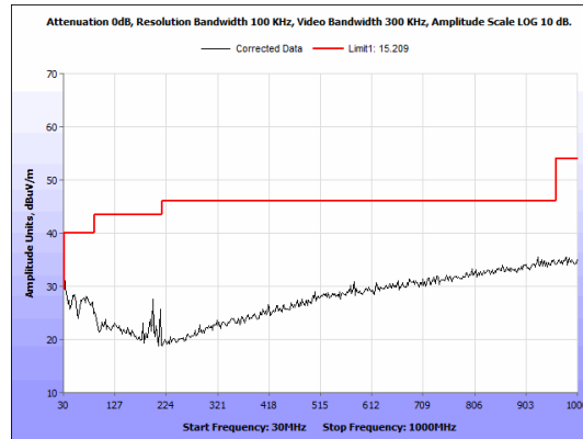
Figure 32: Radiated Emissions, ZigBee 30 MHz - 1 GHz, Mid Channel, Antenna 2
