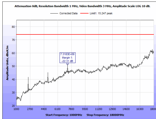
Figure 18: Radiated Emissions, ZigBee, 1GHz - 18GHz Peak, Mid Channel, Antenna 1
