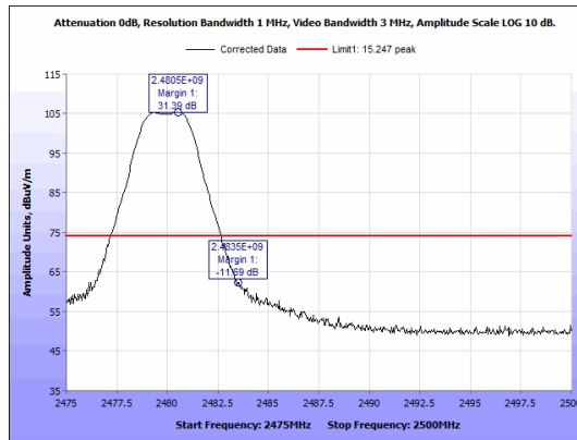
Figure 49: Radiated Emissions, ZigBee High Channel Band Edge, Peak, Antenna 1
