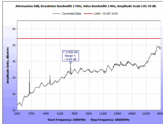
Figure 17: Radiated Emissions, ZigBee, 1GHz - 18GHz, Average, Mid Channel, Antenna 1
