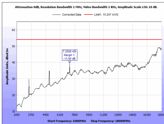
Figure 13: Radiated Emissions, ZigBee, 1GHz - 18GHz, Average, Low Channel, Antenna 1
