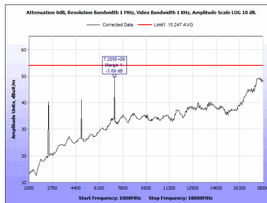
Figure 13: Radiated Emissions, BLE Low Channel, 1GHz - 18GHz, Average, Antenna 1
