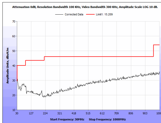
Figure 22: Radiated Emissions, BLE High Channel, 30 MHz - 1 GHz Antenna 1
