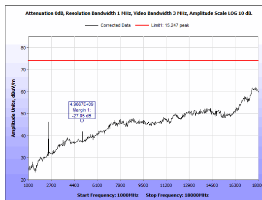
Figure 25: Radiated Emissions, BLE High Channel, 1GHz - 18GHz, Peak, Antenna 1
