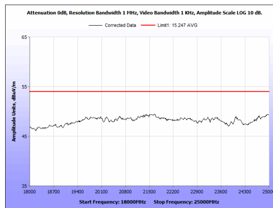
Figure 24: Radiated Emissions, BLE High Channel, 18GHz - 25GHz, Average, Antenna 1
