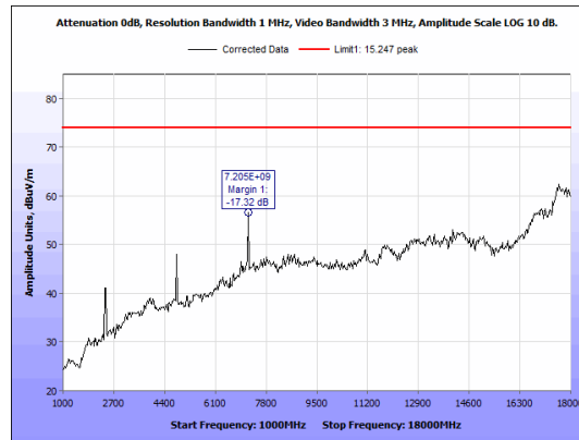
Figure 15: Radiated Emissions, BLE Low Channel, 1GHz - 18GHz, Peak, Antenna 1
