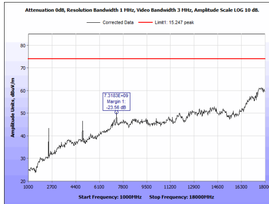
Figure 20: Radiated Emissions, BLE Mid Channel, 1GHz - 18GHz, Peak, Antenna 1
