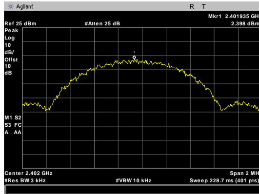
Figure 68: Power Spectral Density, BLE Low Channel
