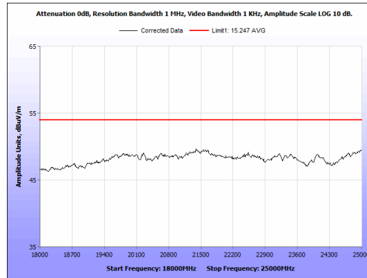
Figure 14: Radiated Emissions, BLE Low Channel, 18GHz - 25GHz, Average, Antenna 1
