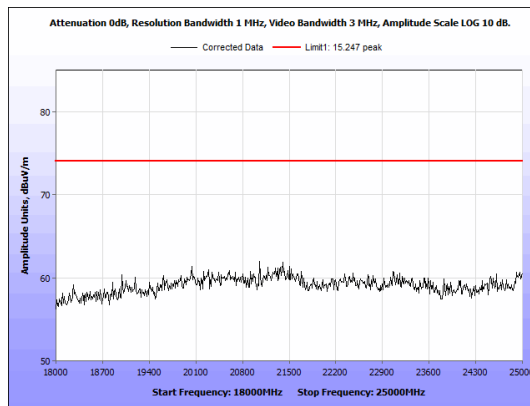
Figure 21: Radiated Emissions, BLE Mid Channel, 18GHz - 25GHz, Peak, Antenna 1
