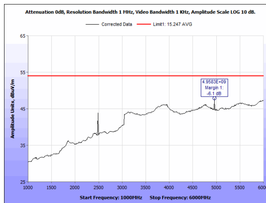
Figure 43: Radiated Emissions, BLE High Channel, 1GHz - 6 GHz, Average, Antenna 2
