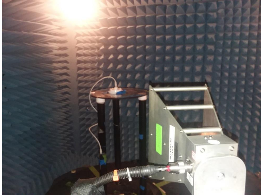
Figure 3: Radiated Emissions, Peak, High Channel, 1 GHz – 18 GHz, Test Setup
