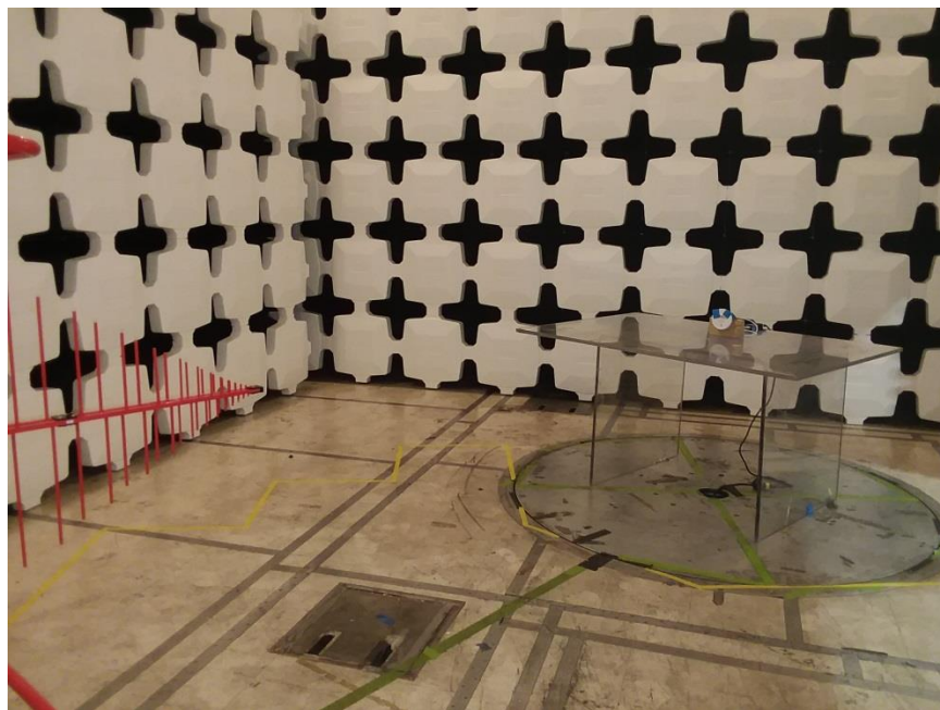
Figure 2: Radiated Emissions, Peak, High Channel, 30MHz – 1GHz, Test Setup
